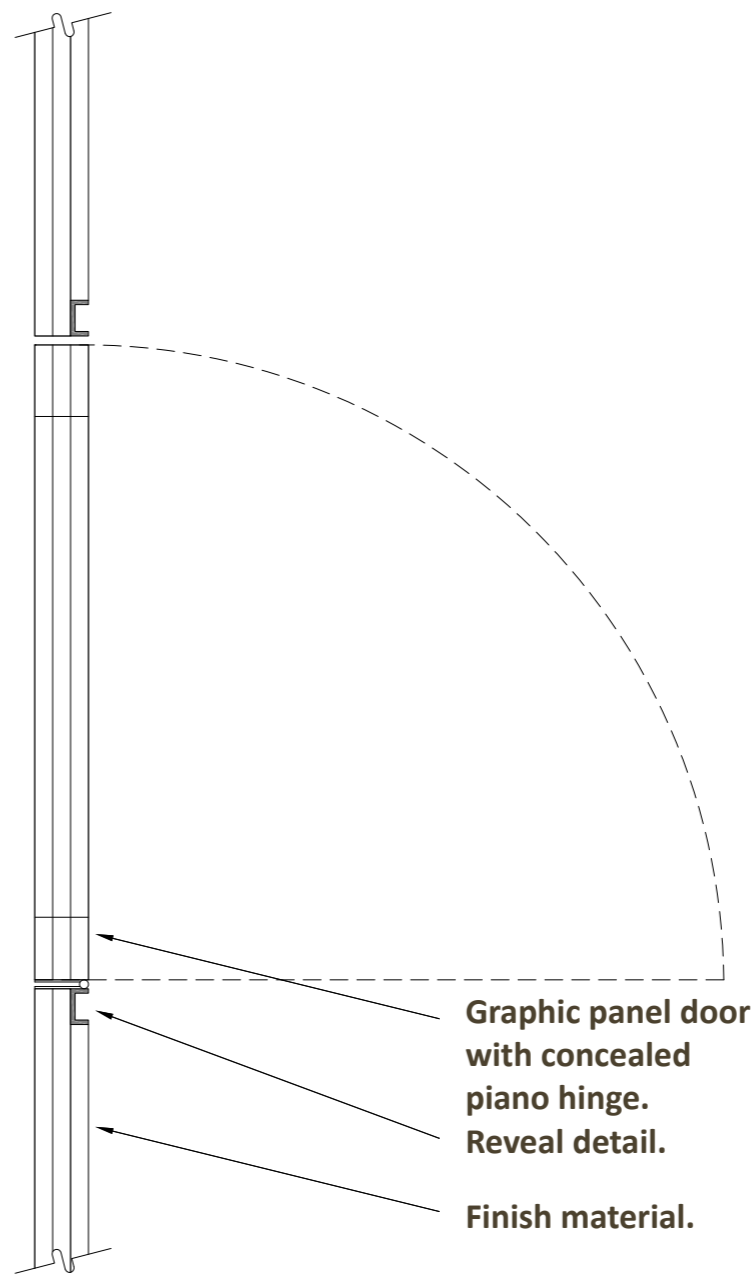
GRAPHIC FRAME DETAIL
