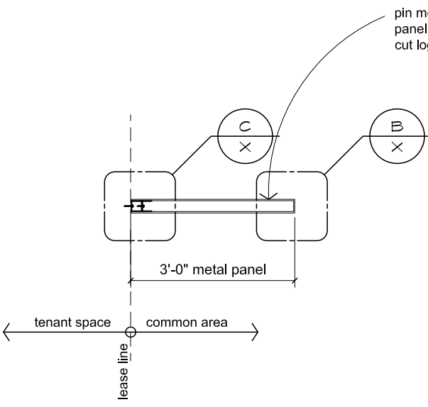
A Plan Detail scale: 1/2"=1'-0"
