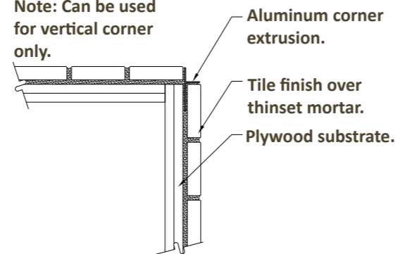
CORNER DETAIL
