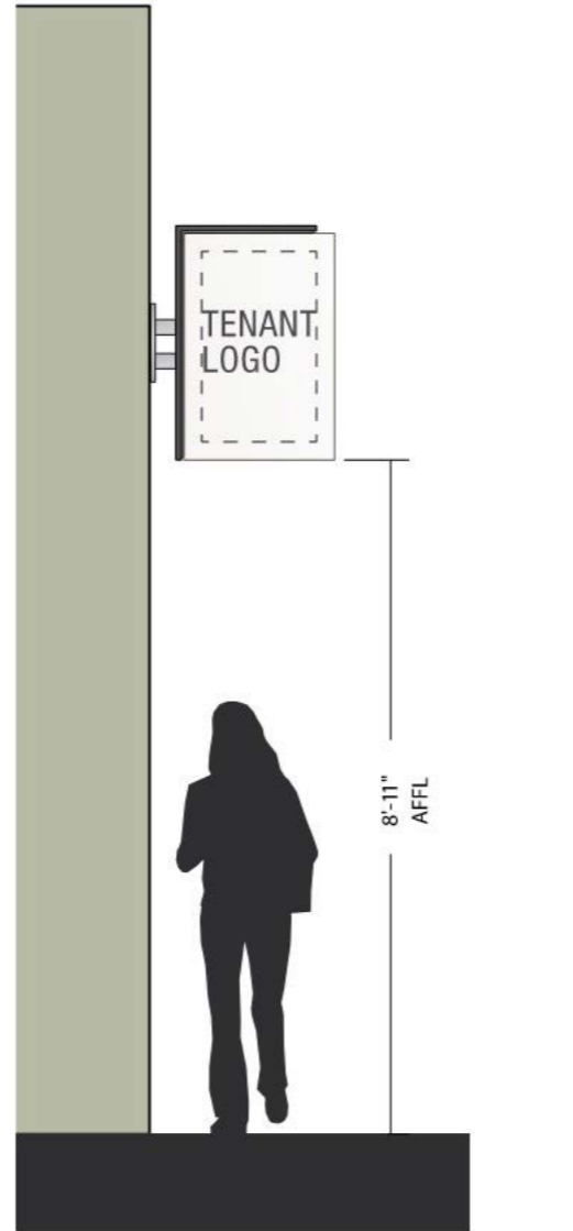
2 Context Elevation | Vertical Tenant Blade Scale: 1/2" = 1'-0"
