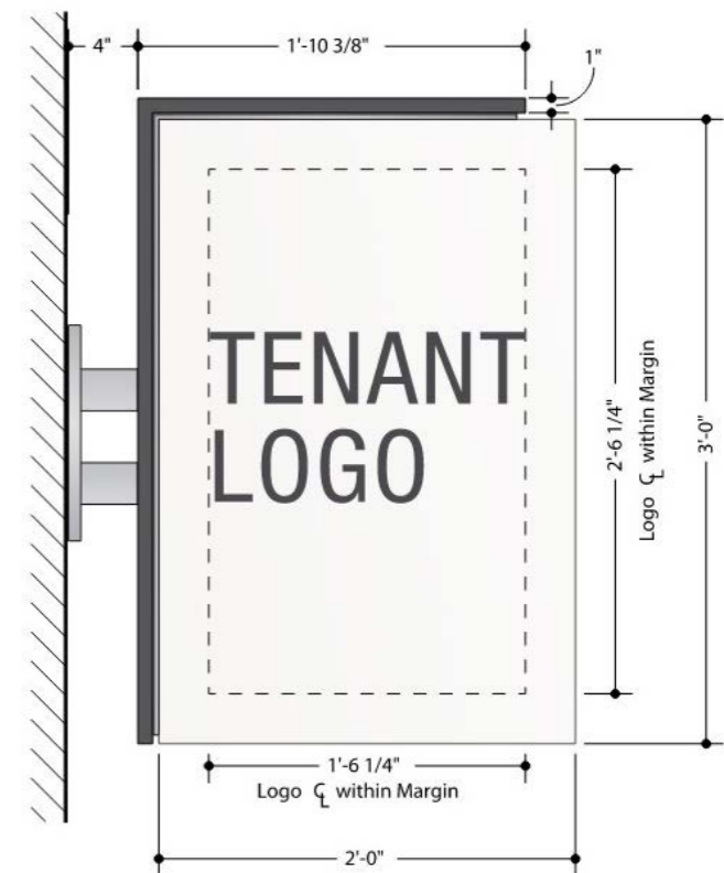
2 Elevation | Vertical Tenant Blade Scale: 1 1/2" = 1'-0"
