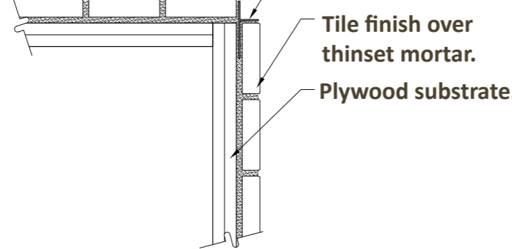
CORNER DETAIL
