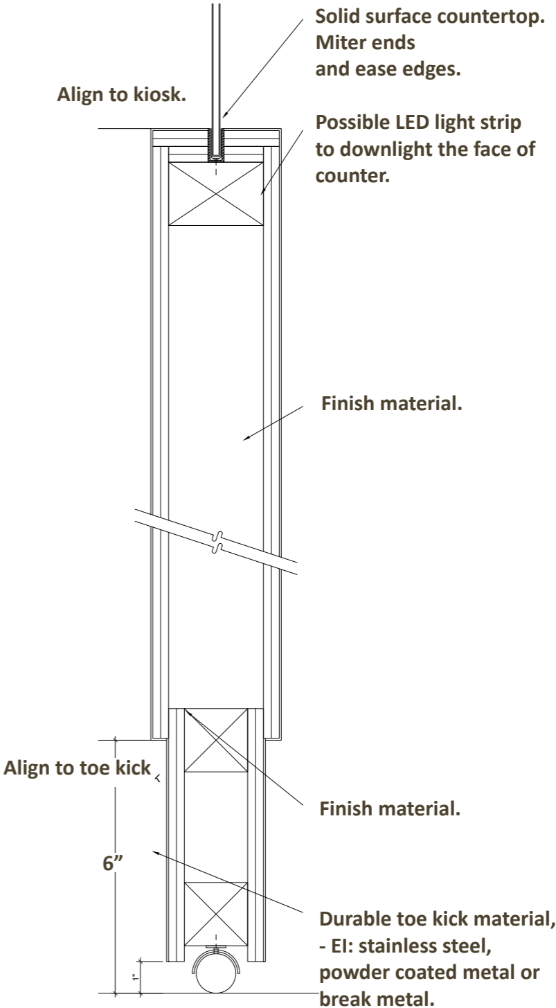
GATE DETAIL
