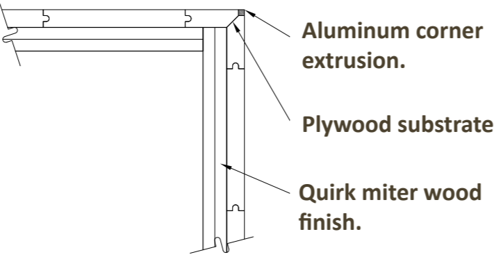
CORNER DETAIL
