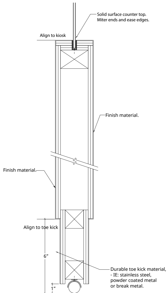
GATE DETAIL
