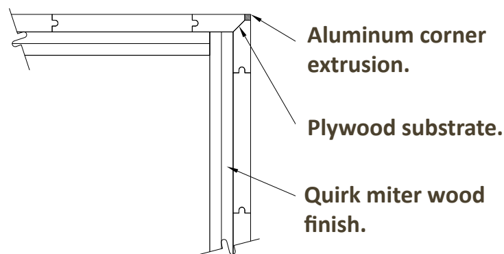
CORNER DETAIL
