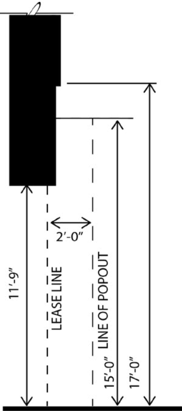
SECTION
