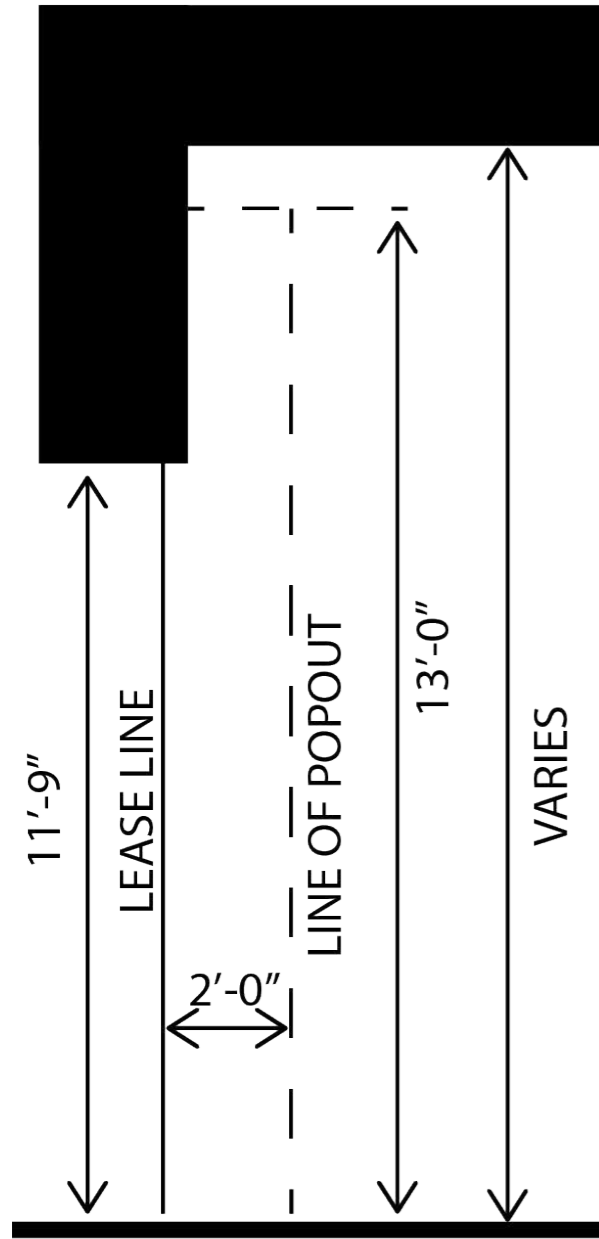
SECTION
