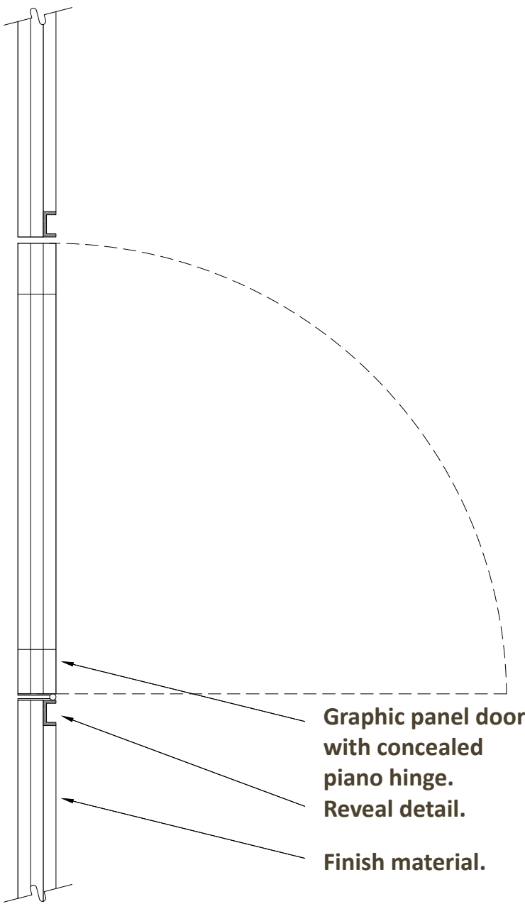
GRAPHIC FRAME DETAIL
