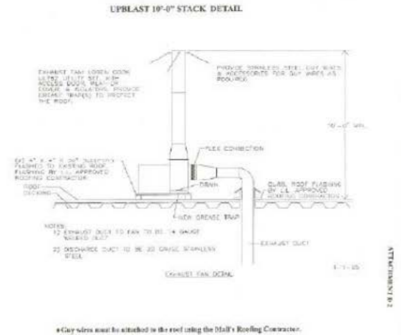
Upblast Stack Detail
