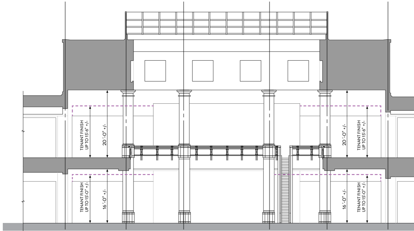
DETAIL 'CENTER COURT'
