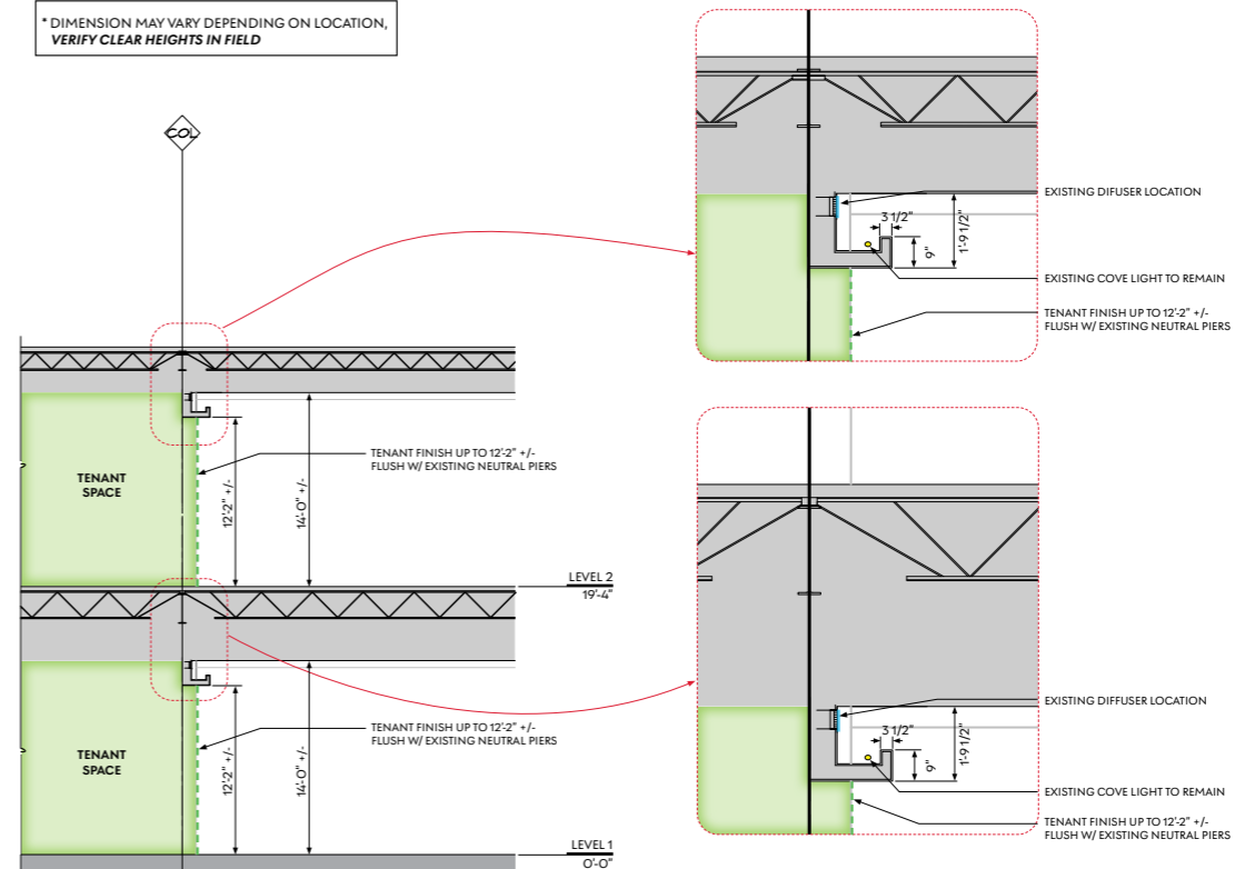
DETAIL 'F'- ENTRY 1 AND 5 WING
