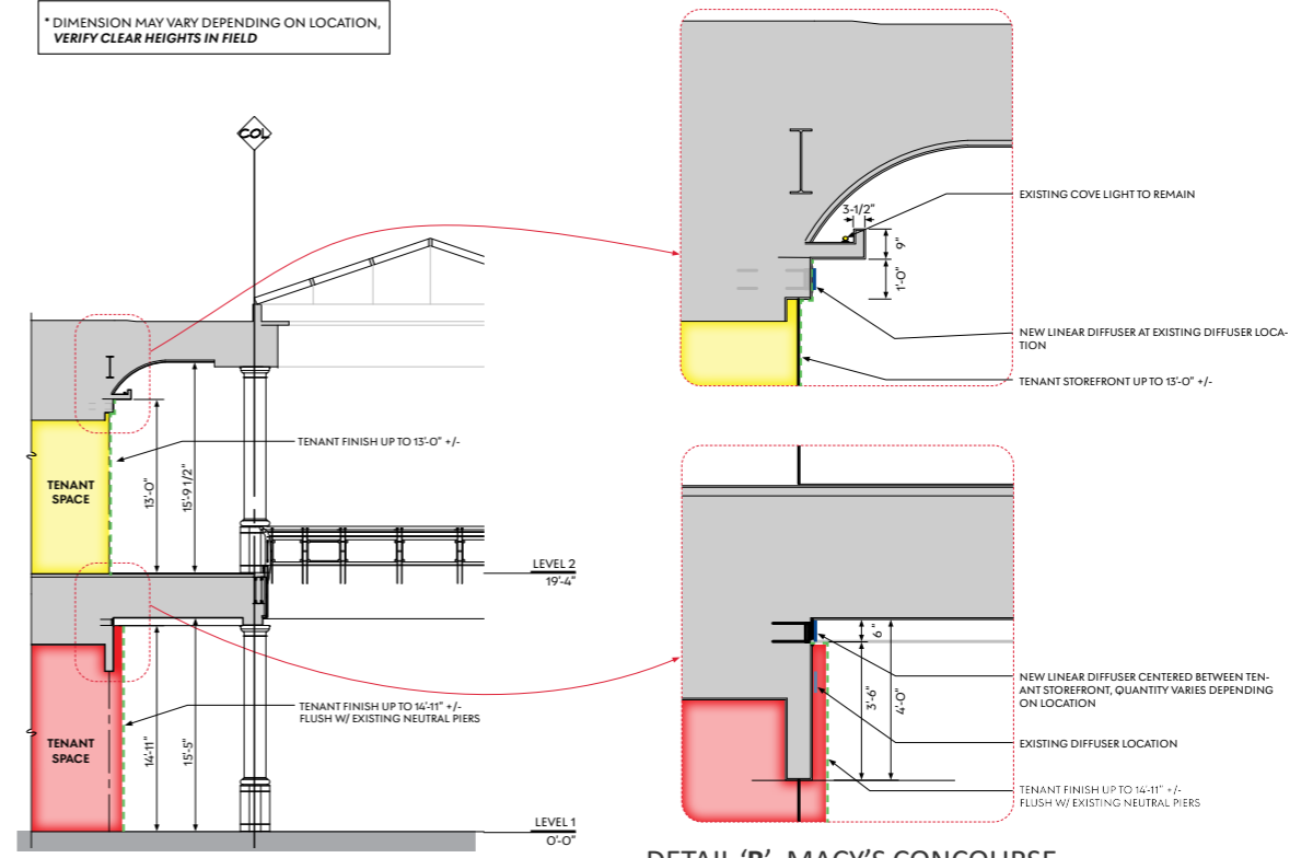
DETAIL 'B'- MACY'S CONCOURSE
