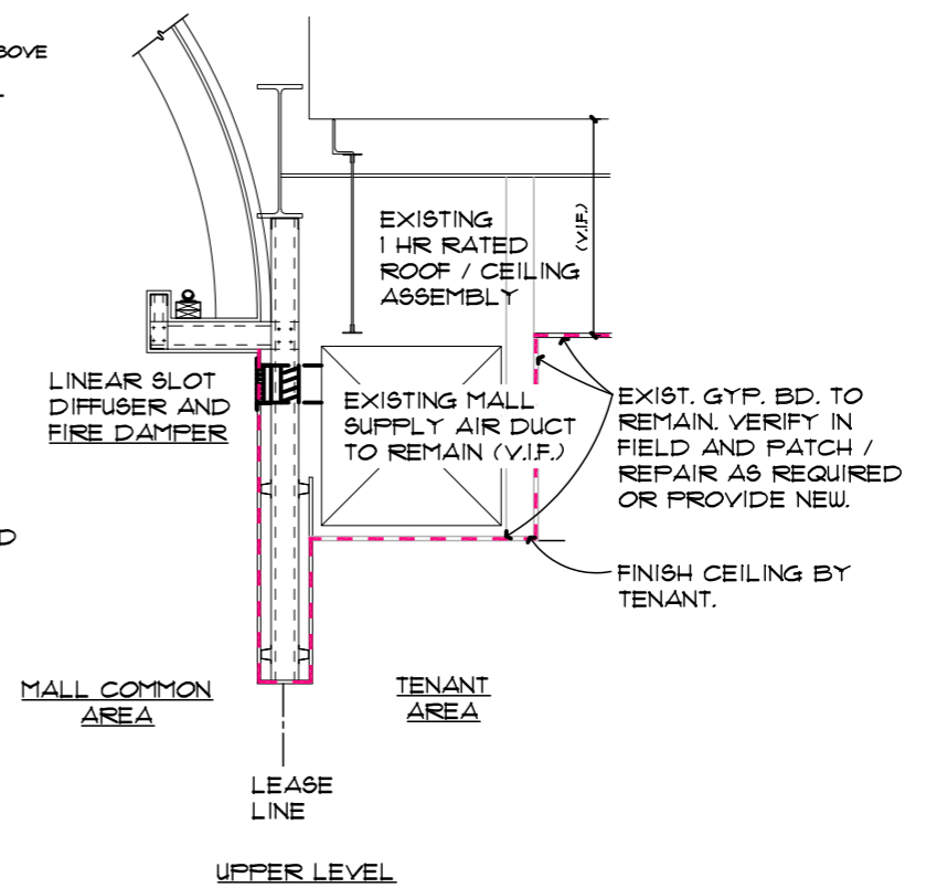
CONDITION #2 FIRE SEPARATION BELOW DUCT (VERIFY IN FIELD WHERE OCCURS)
