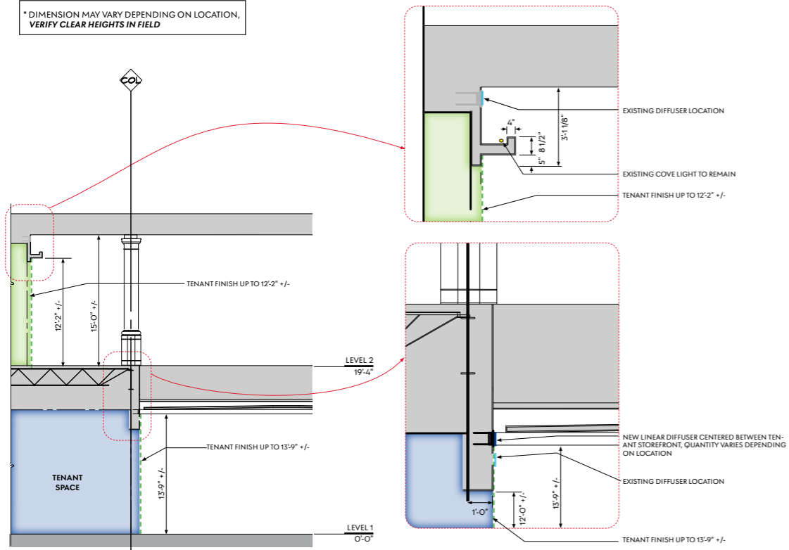
DETAIL 'E'- ENTRY 3 AND BELK MEN'S WING
