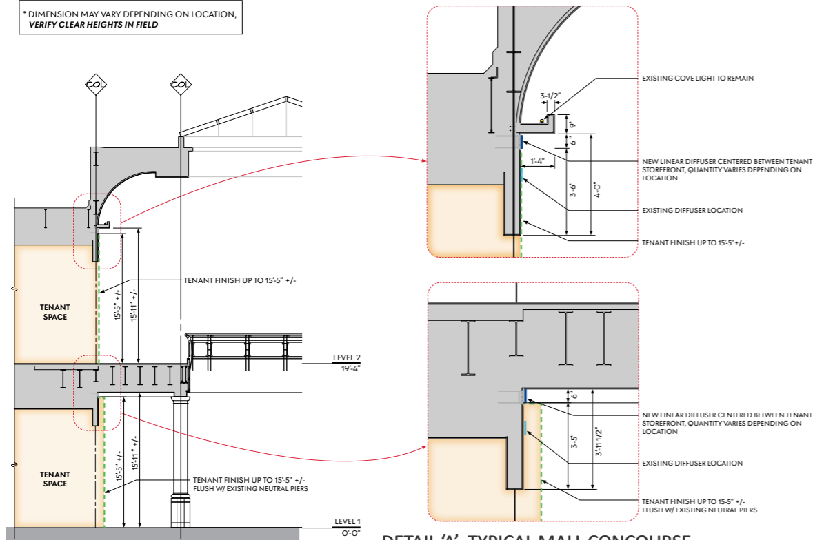
DETAIL 'A'- TYPICAL MALL CONCOURSE
