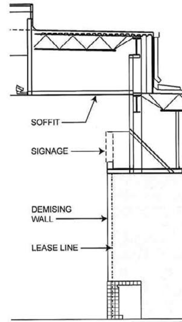
SECTION
