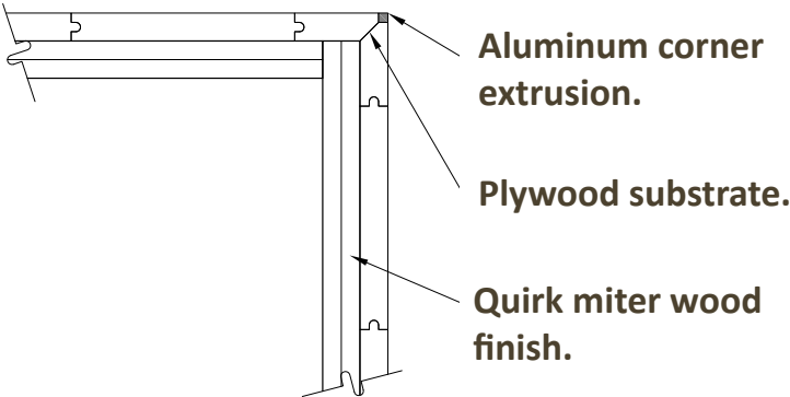
CORNER DETAIL
