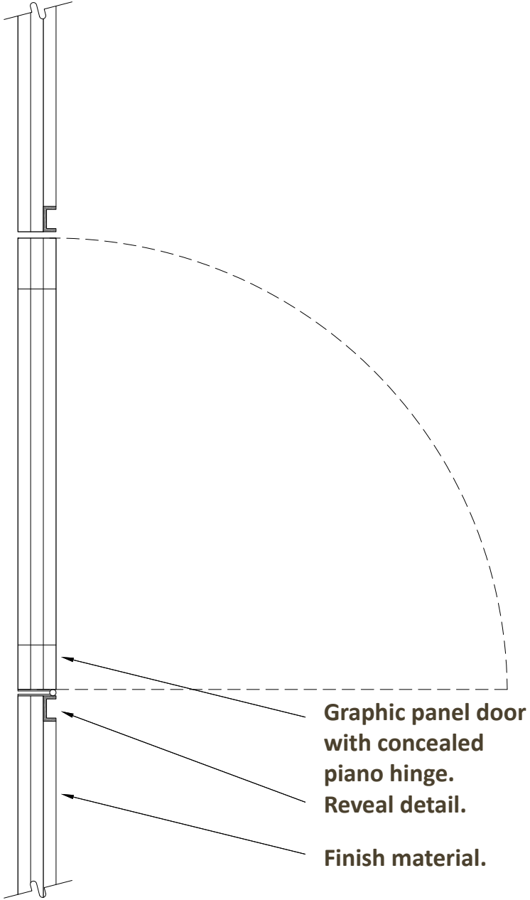
GRAPHIC FRAME DETAIL
