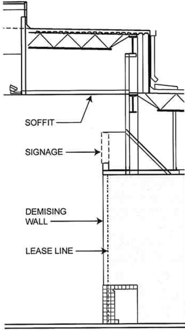
SECTION
