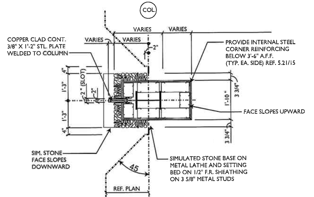
02 FEATURE COLUMN PLAN DETAIL
