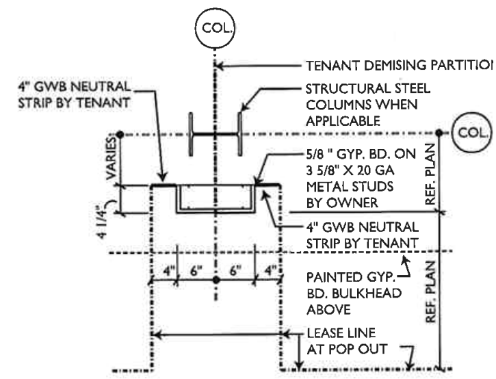
04 TYPICAL NEUTRAL PIER
