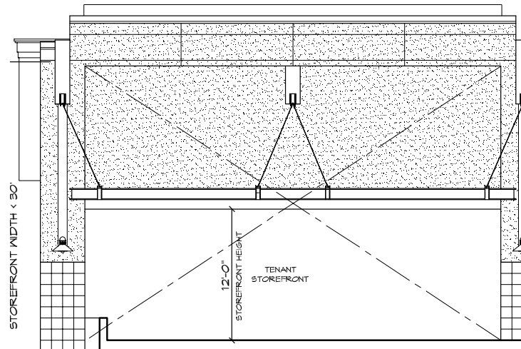
South-Facing Elevation
