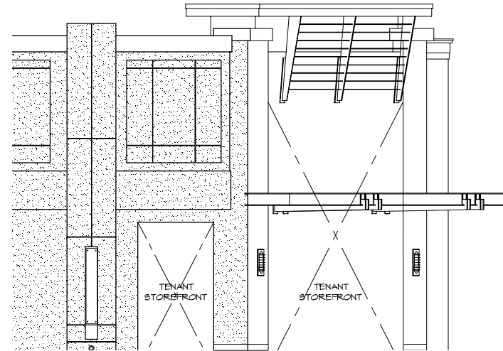
Northwest-Facing Elevation
