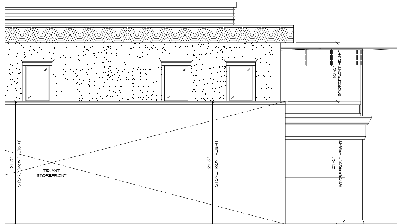
North-Facing Elevation
