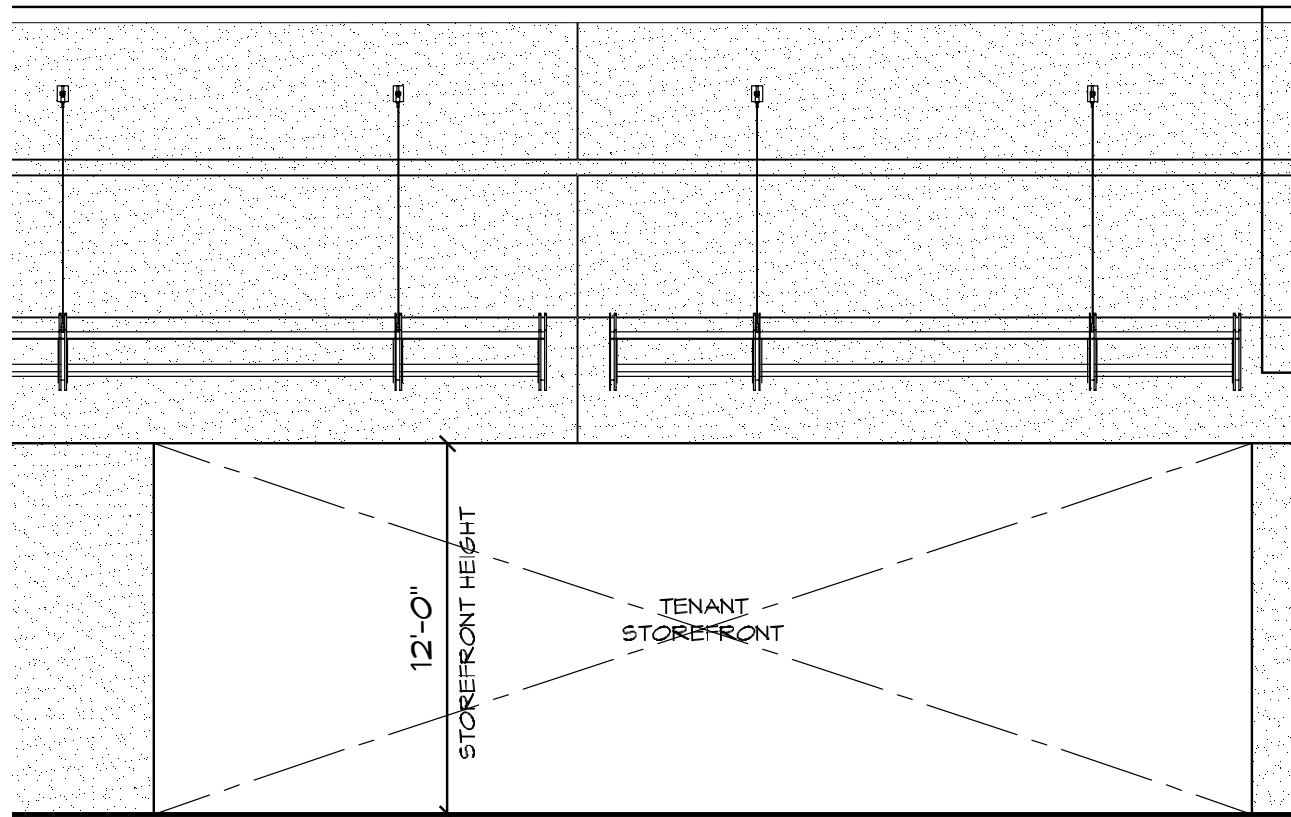
North-Facing Elevation
