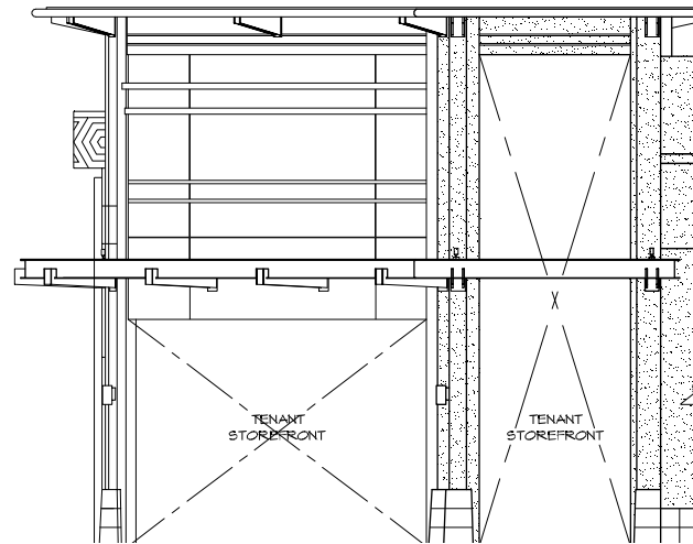
Northeast-Facing Elevation
