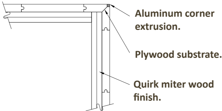
CORNER DETAIL
