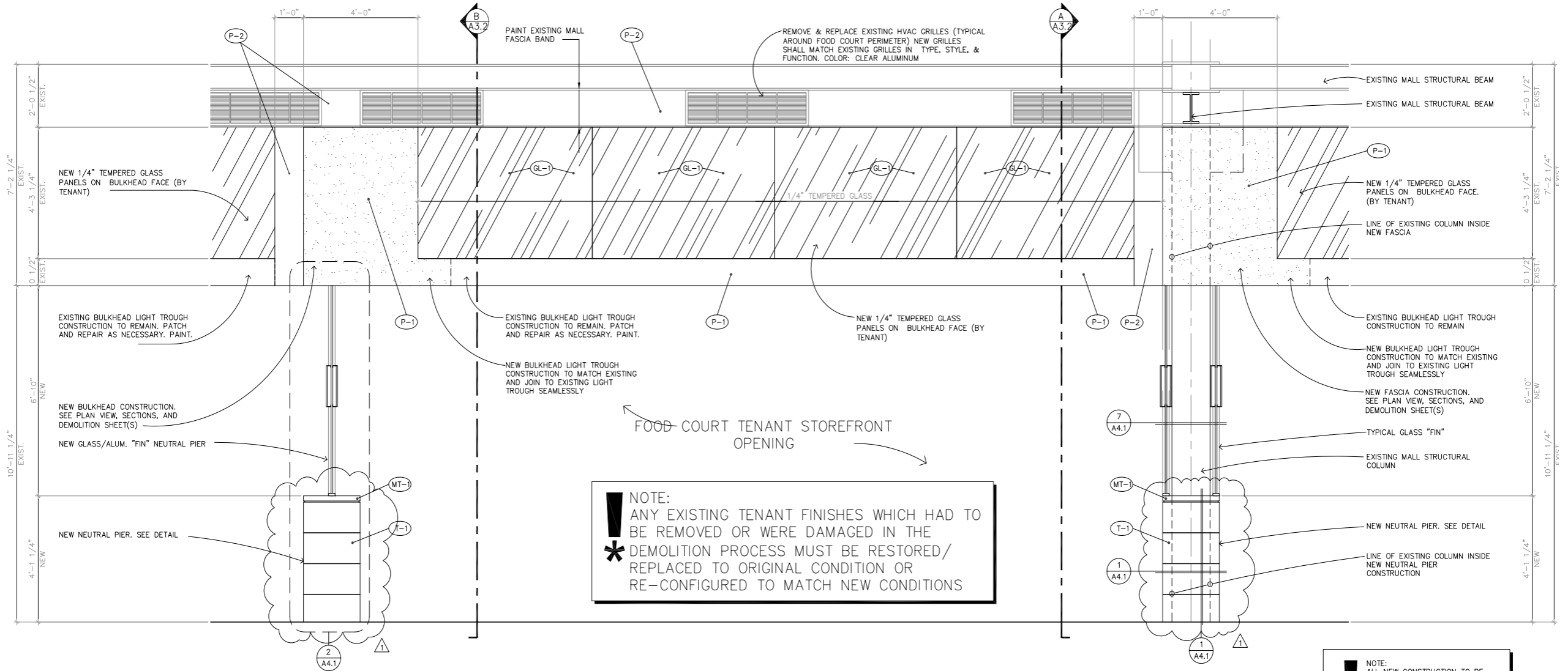
(A) ELEVATION – NEW (TYPICAL @ EACH FOOD COURT TENANT) SCALE: 1/2" = 1'-0"
