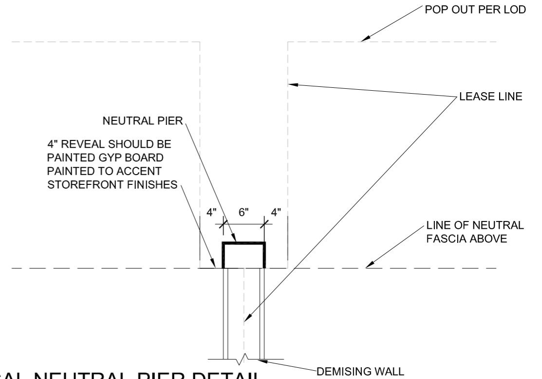
TYPICAL NEUTRAL PIER DETAIL
