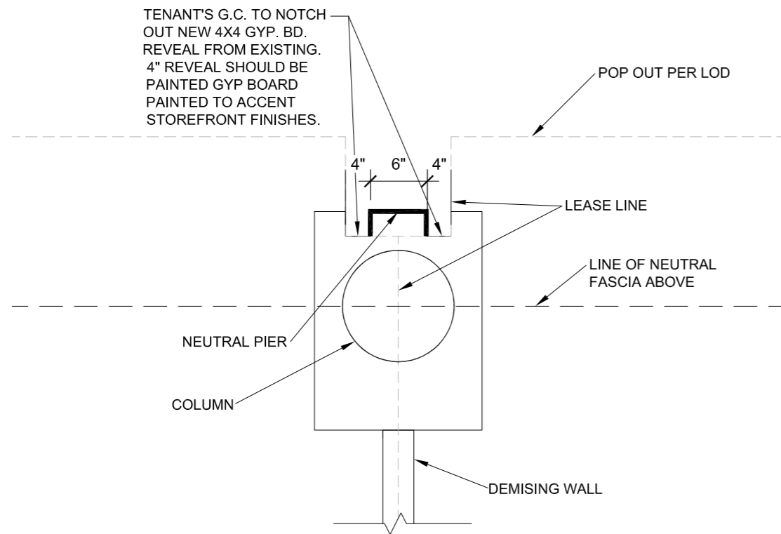
TYPICAL NEUTRAL PIER DETAIL @ COLUMN
