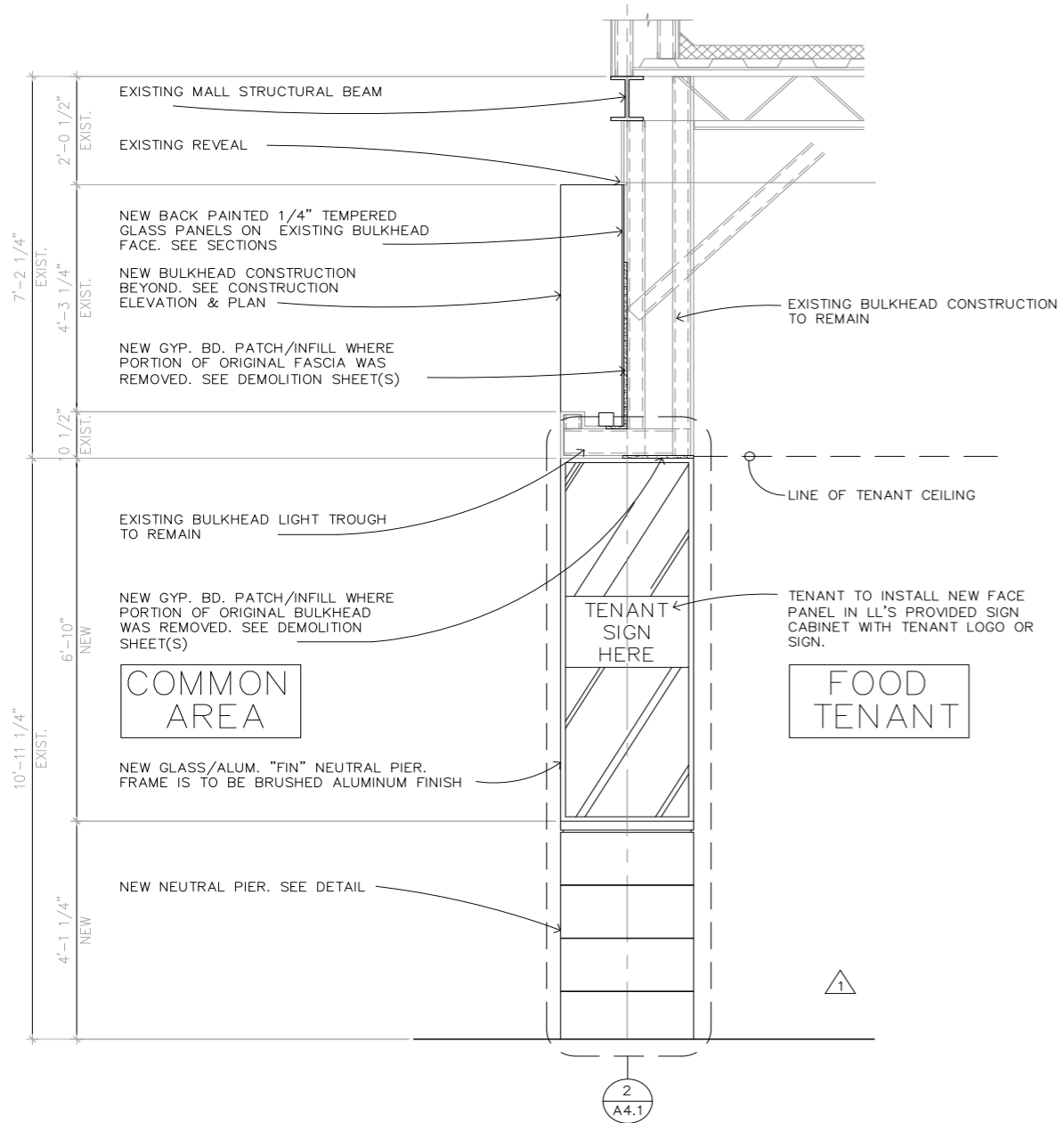
B TYPICAL SECTION — NEW
