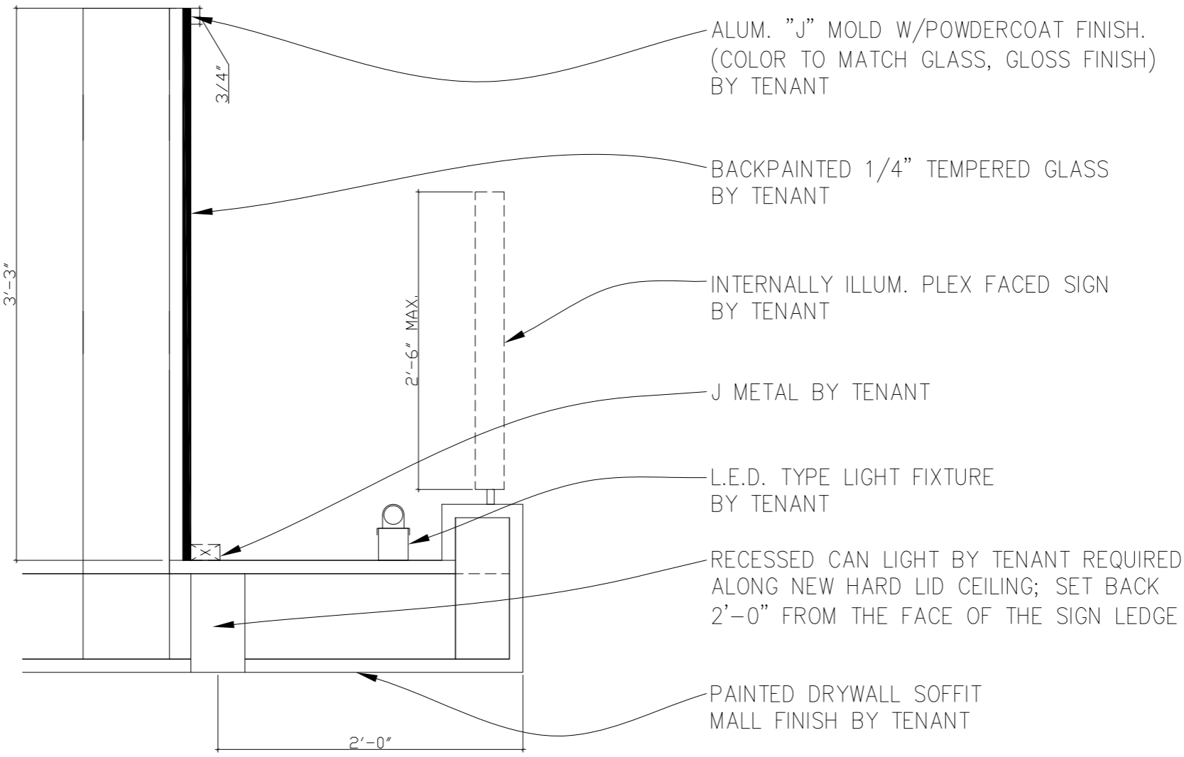
BACK PAINTED GLASS DETAIL N.T.S.
