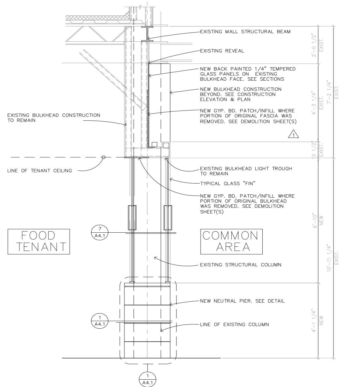
A TYPICAL SECTION — NEW
