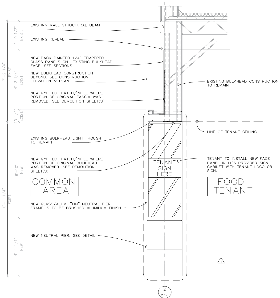
B TYPICAL SECTION — NEW
