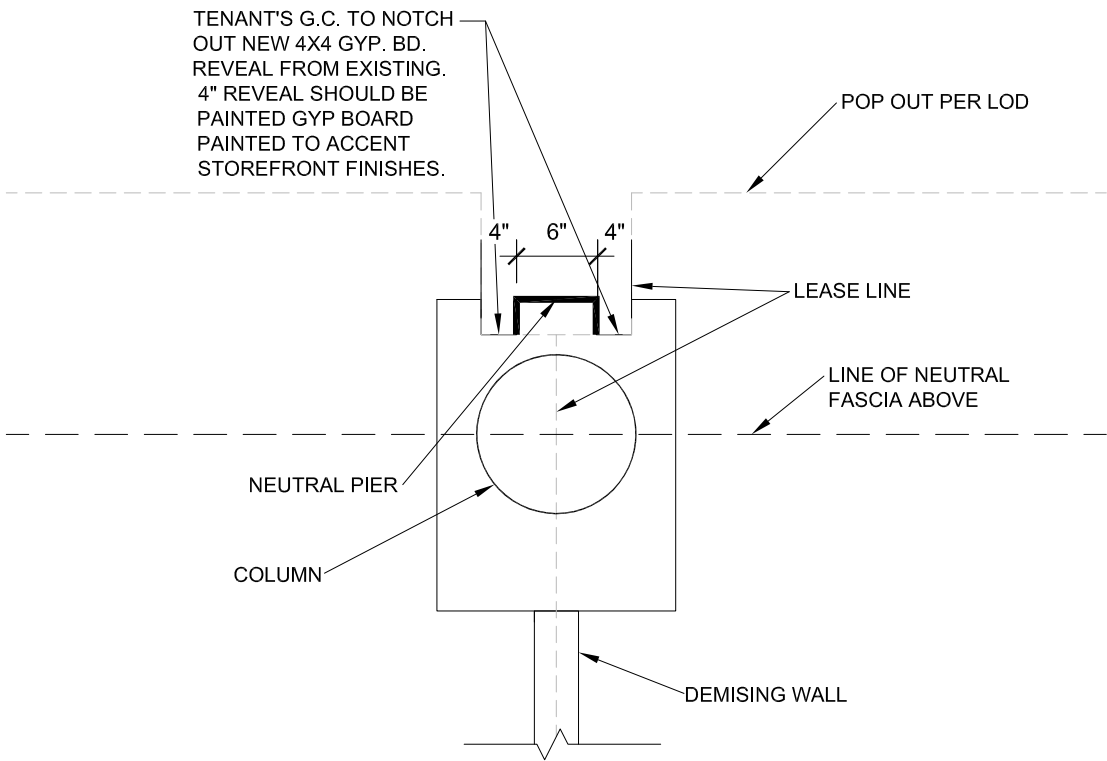
TYPICAL NEUTRAL PIER DETAIL @ COLUMN *CONTACT MALL T.C. FOR MORE INFORMATION N.T.S.
