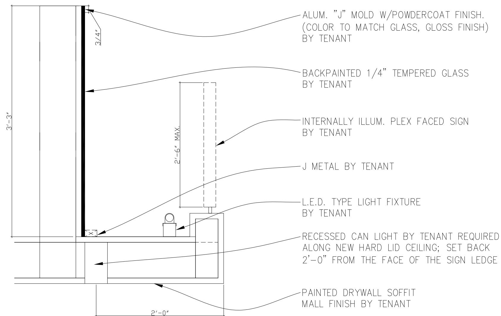
BACK PAINTED GLASS DETAIL N.T.S.
