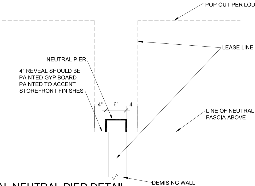
TYPICAL NEUTRAL PIER DETAIL *CONTACT MALL T.C. FOR MORE INFORMATION N.T.S.
