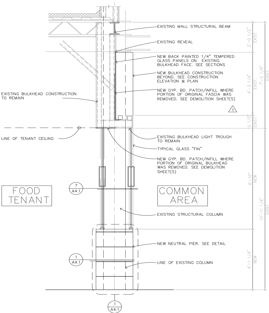
A TYPICAL SECTION — NEW
