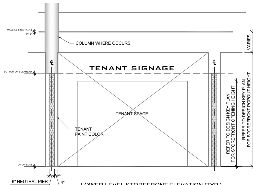
LOWER LEVEL STOREFRONT ELEVATION (TYP.) NOT TO SCALE - TENANT TO VERIFY ALL EXISTING CONDITIONS
