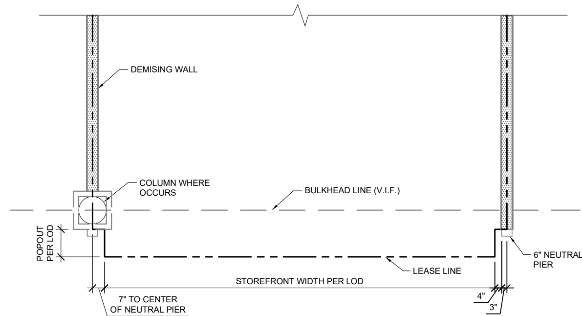
LOWER LEVEL PLAN (TYP.) NOT TO SCALE - TENANT TO VERIFY ALL EXISTING CONDITIONS
