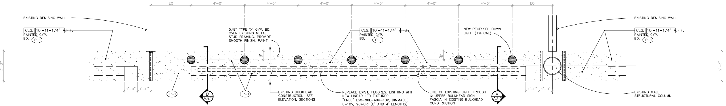
1 PARTIAL FLOOR PLAN – NEW (TYPICAL @ EACH FOOD COURT TENANT) SCALE: 1/2" = 1'-0"
