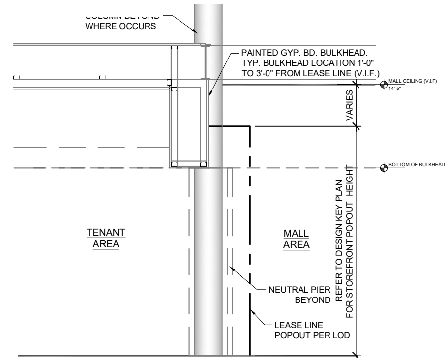
LOWER LEVEL STOREFRONT SECTION (TYP.) NOT TO SCALE - TENANT TO VERIFY ALL EXISTING CONDITIONS
