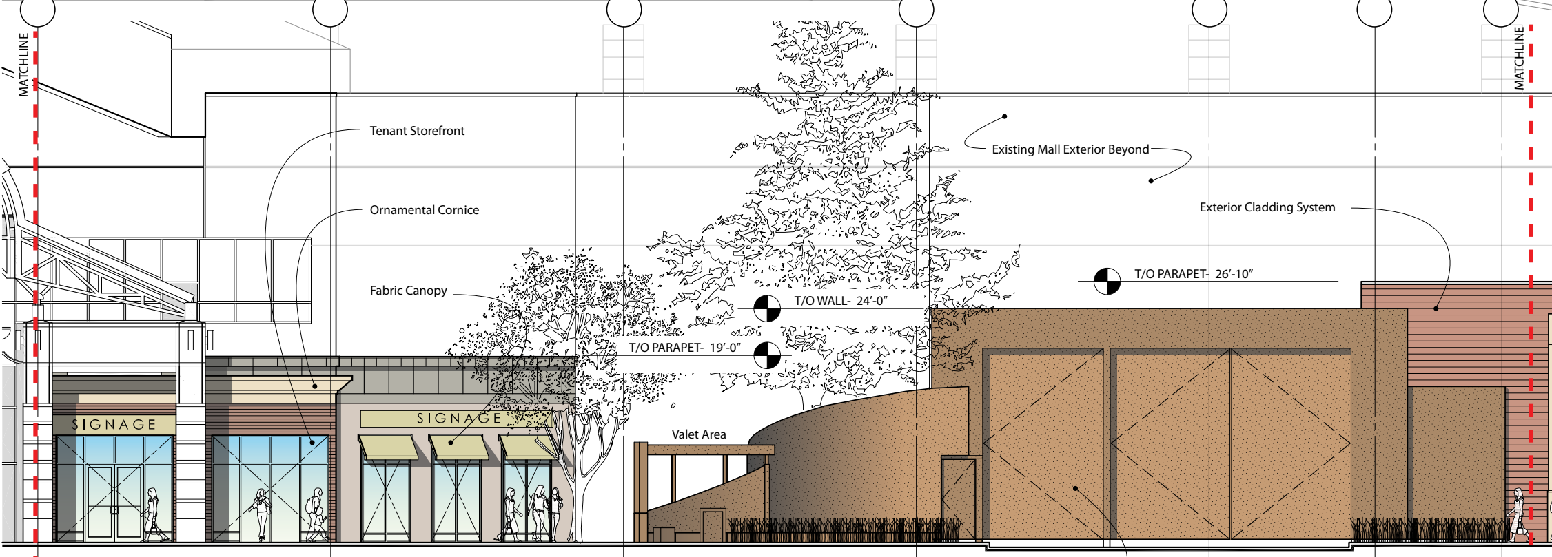
1 Elevation- Area 02 Scale: 1/16" = 1'-0"
