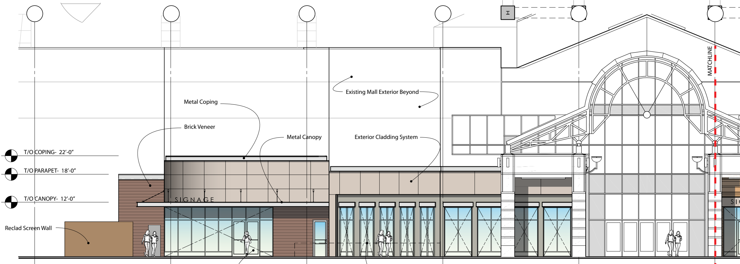
1 Elevation- Area 01 Scale: 1/16" = 1'-0"
