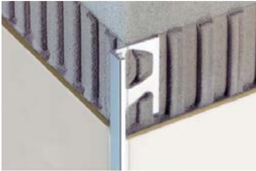
SCHLUTER "JOLLY" STAINLESS STEEL OUTSIDE WALL CORNER PROTECTOR
