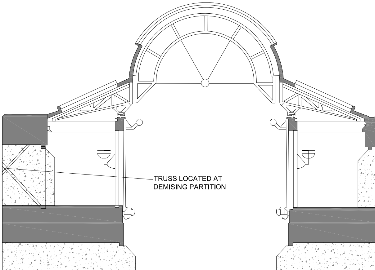
TYP. SECTION AT EAST MALL
