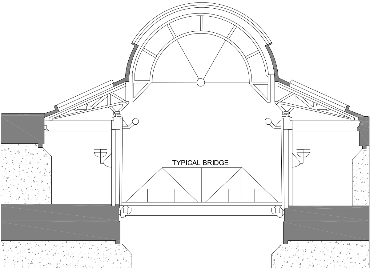
TYP. SECTION AT WEST MALL
