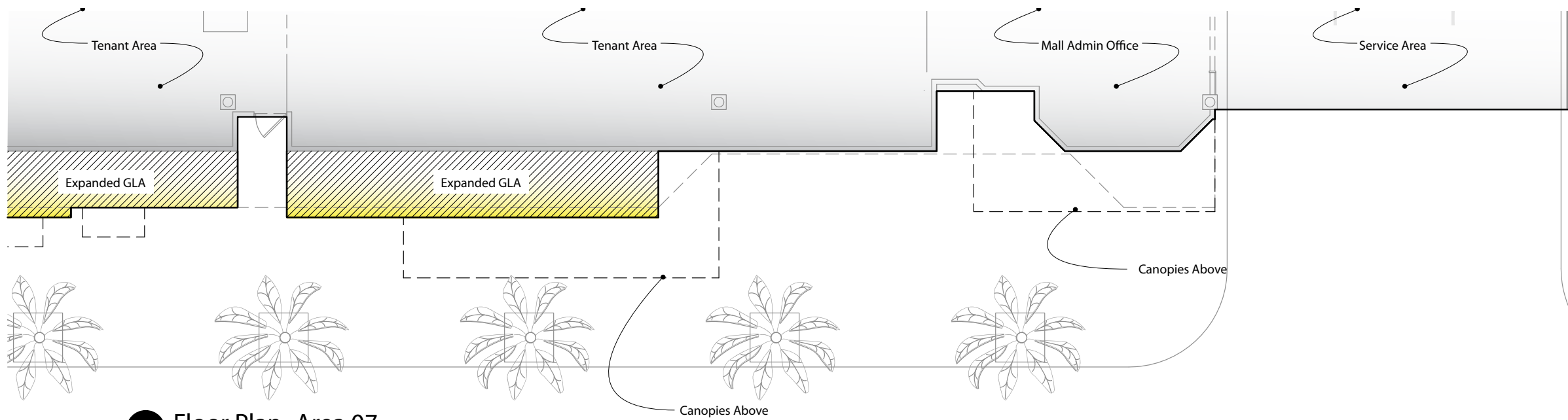
2 Floor Plan- Area 07 Scale: 1/16" = 1'-0"
