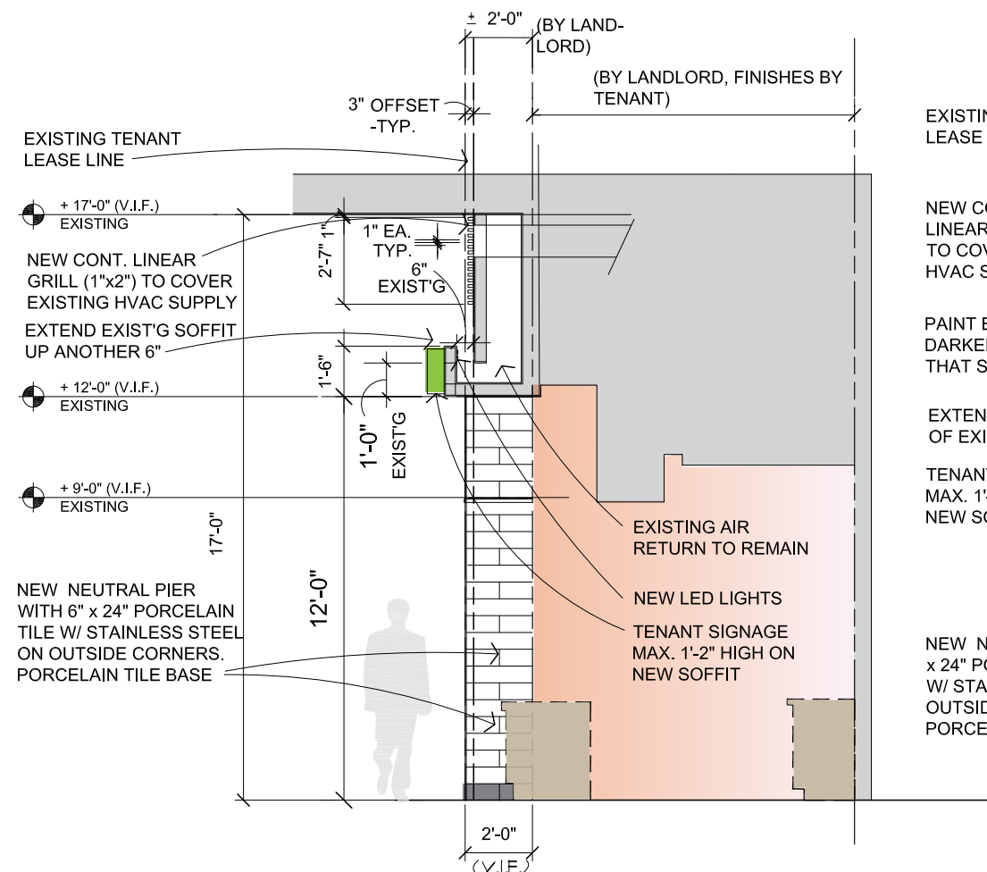
FOOD COURT TENANT NEUTRAL PIER - SIDE ELEVATION SCALE: 1/4" = 1'-0"
