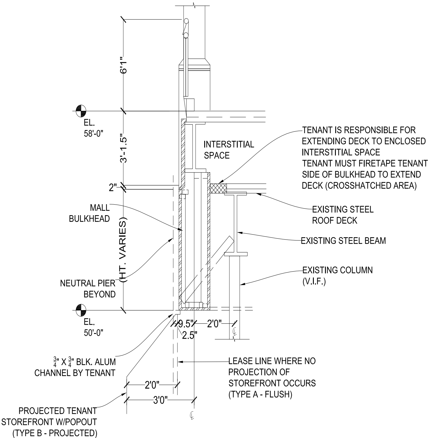
BULKHEAD DETAIL TYP. THROUGHOUT GROUND LEVEL
