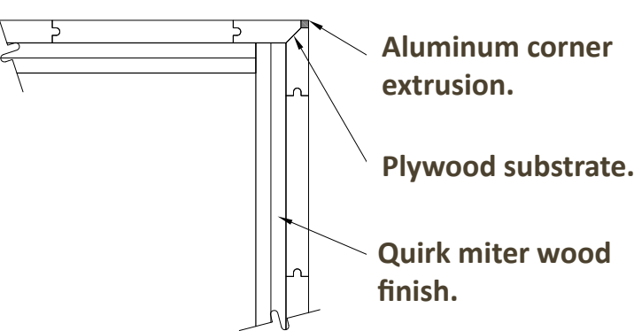
CORNER DETAIL
