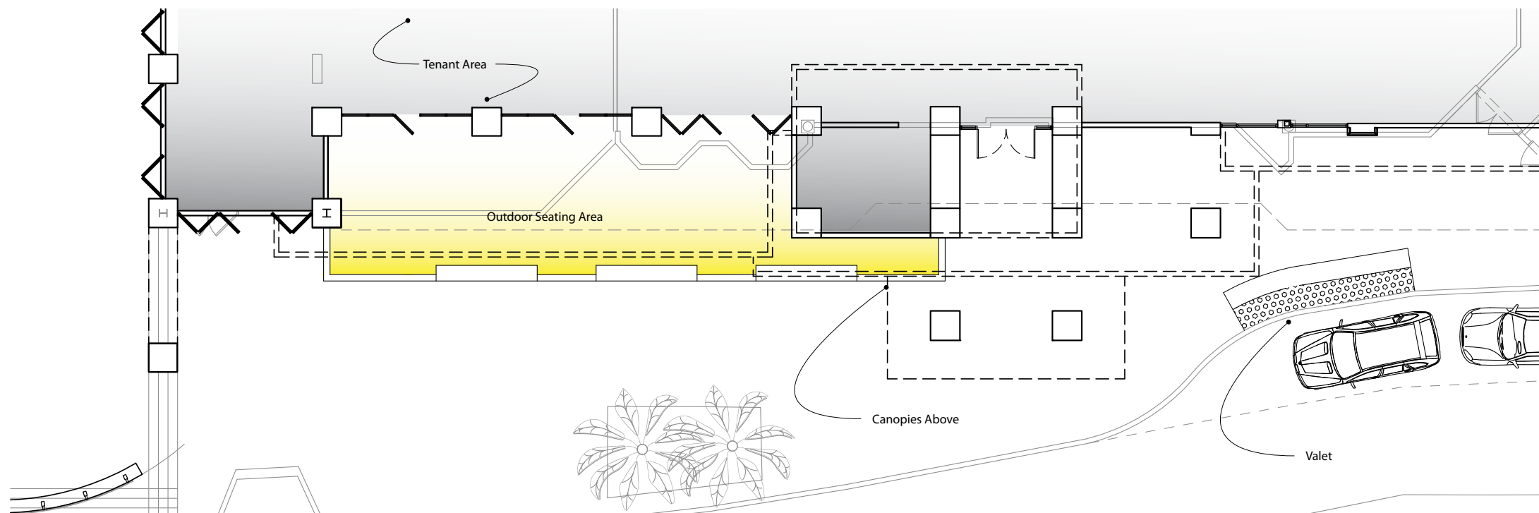
2 Floor Plan- Area 04 Scale: 1/16" = 1'-0"
