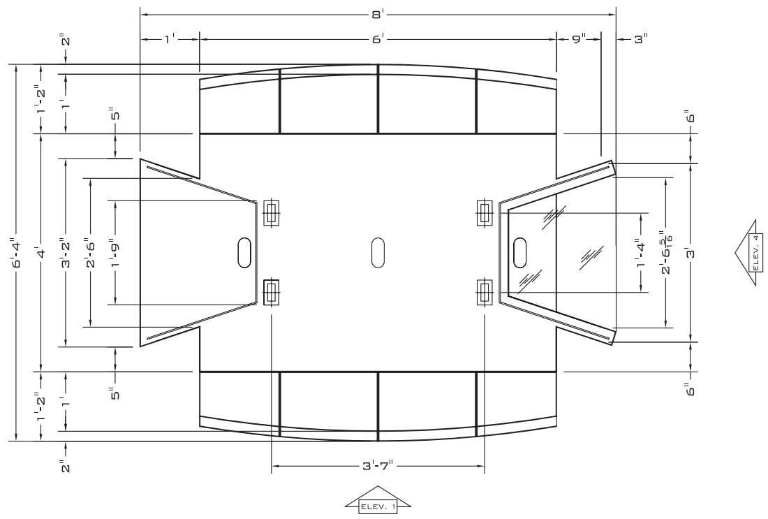
PLAN PLAN @ COUNTER TOP 1 SCALE: 3/4"=1'-0"
