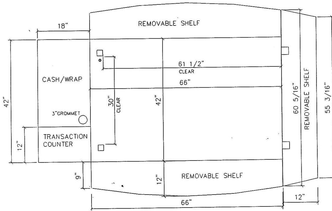
PLAN - COUNTER TOP/COUNTER SHELVES
