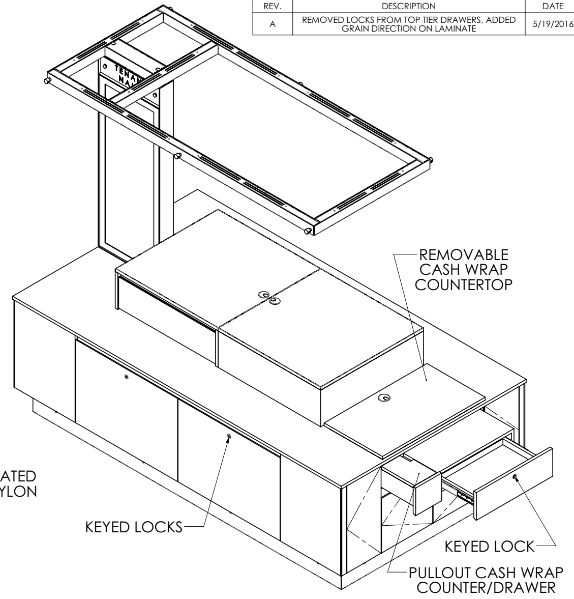
CASH WRAP ISOMETRIC VIEW
