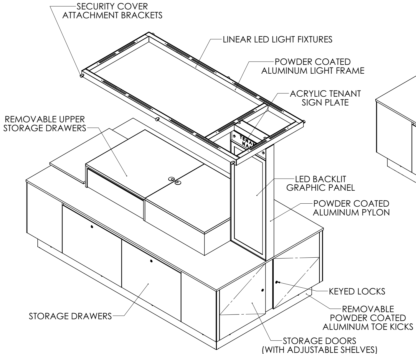
RETAIL ISOMETRIC VIEW
