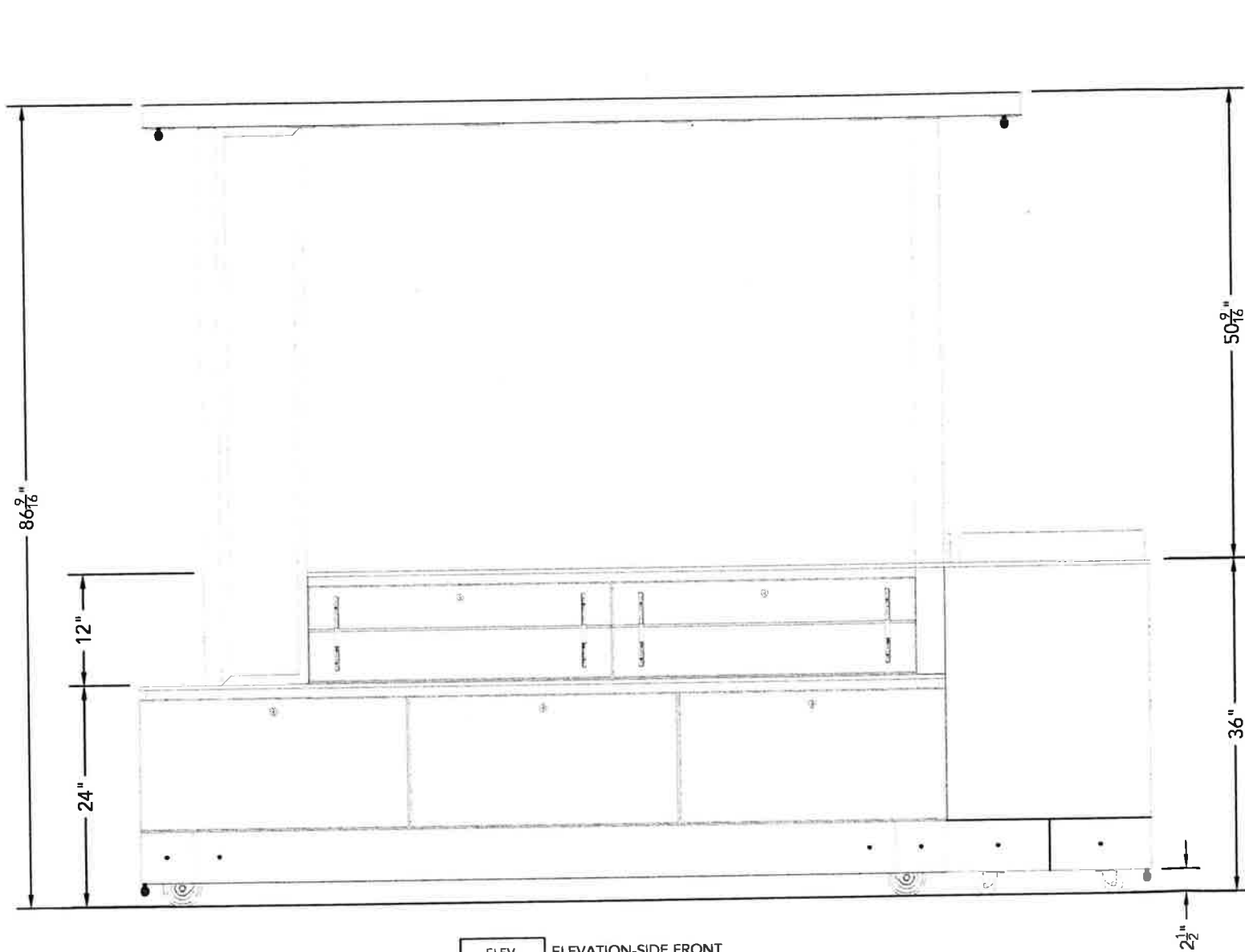
ELEV. ELEVATION-SIDE FRONT 2 SCALE: 3/4"=1'-0"
