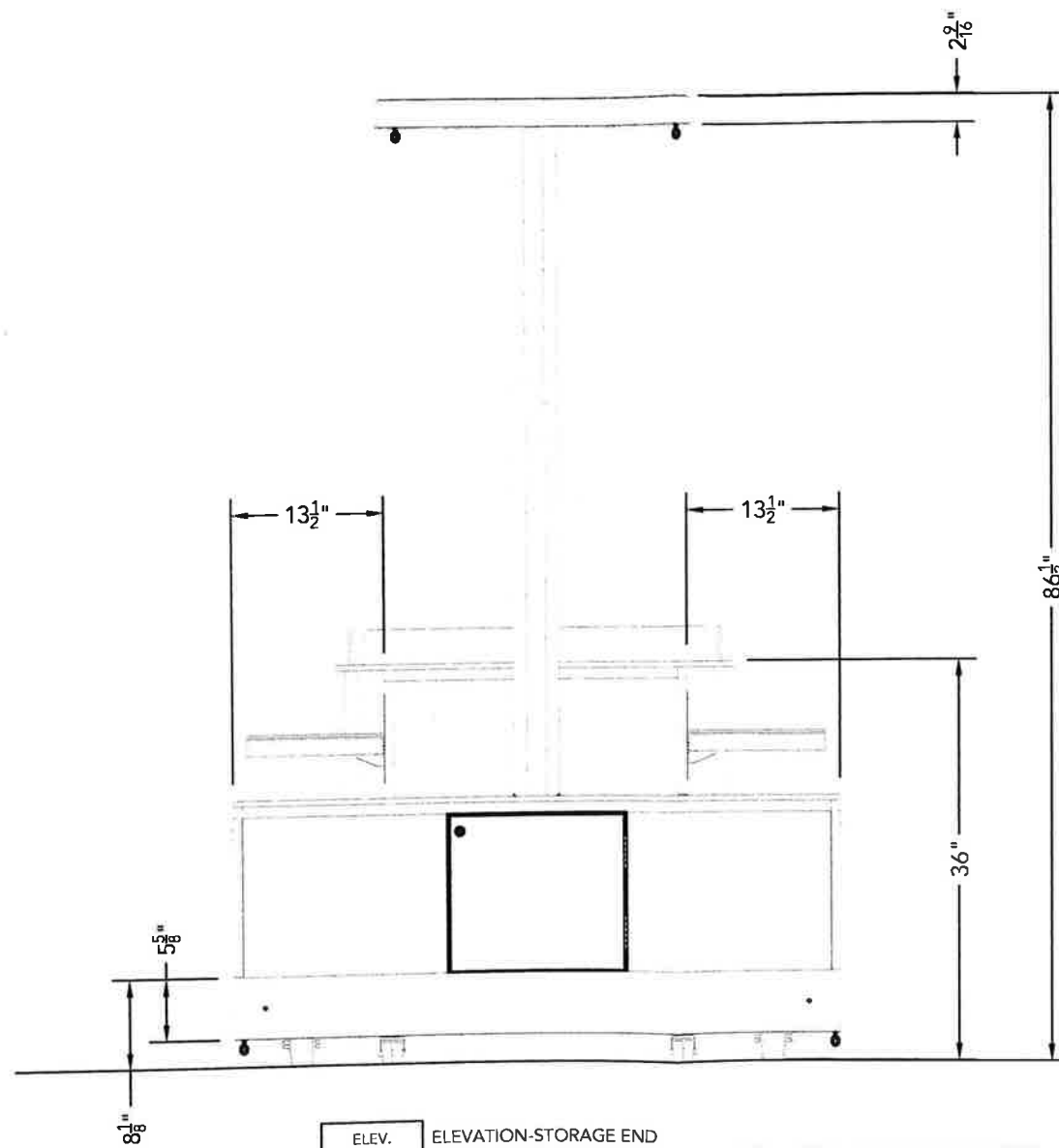
ELEV. ELEVATION-STORAGE END 4 SCALE: 3/4"=1'-0"
