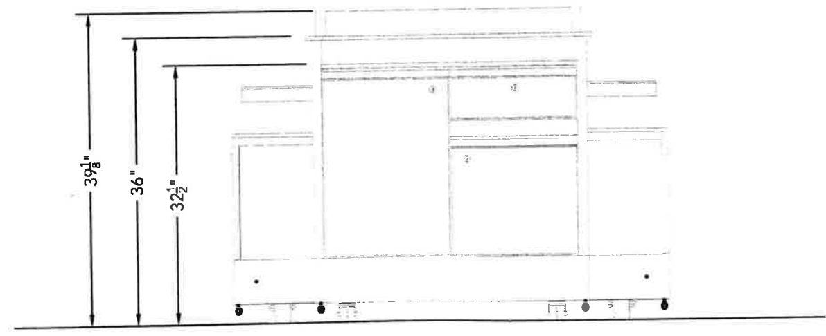
ELEV. ELEVATION-CASH STAND 3 SCALE: 3/4"=1'-0"
