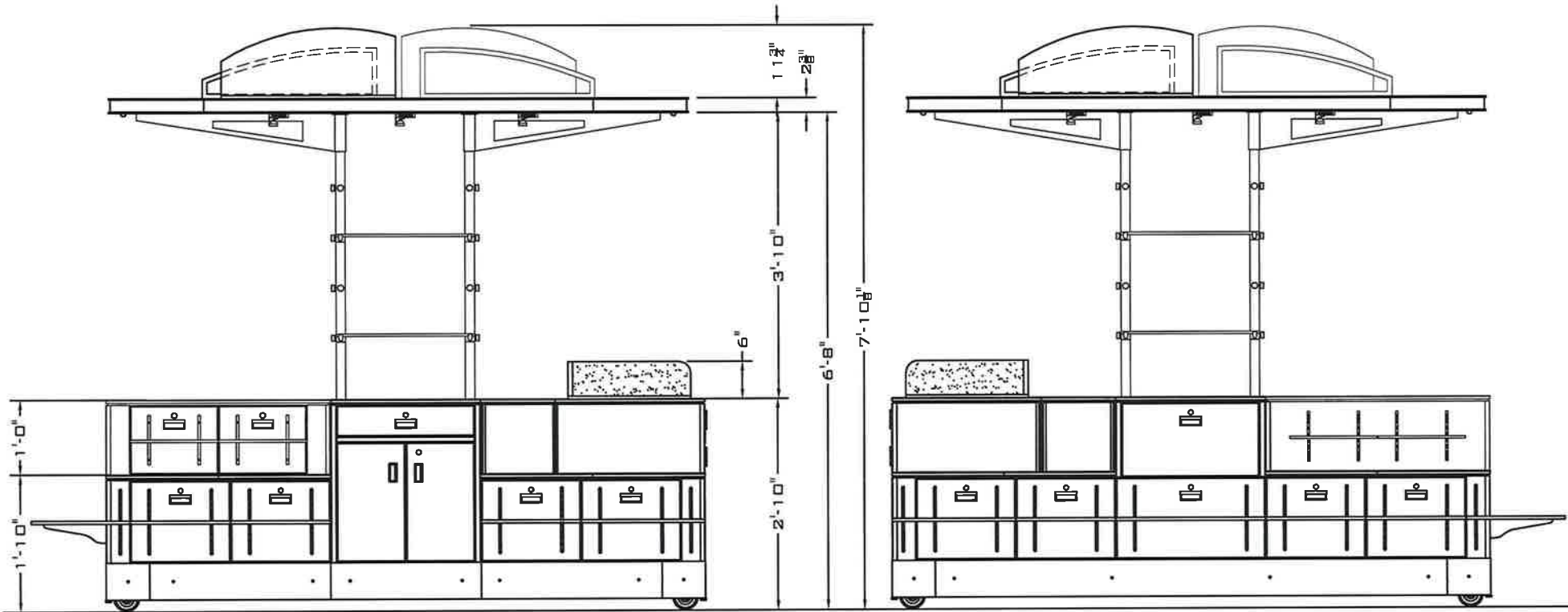
ELEV. 2 ELEVATION-SIDE REAR SCALE: 3/4"=1'-0"
