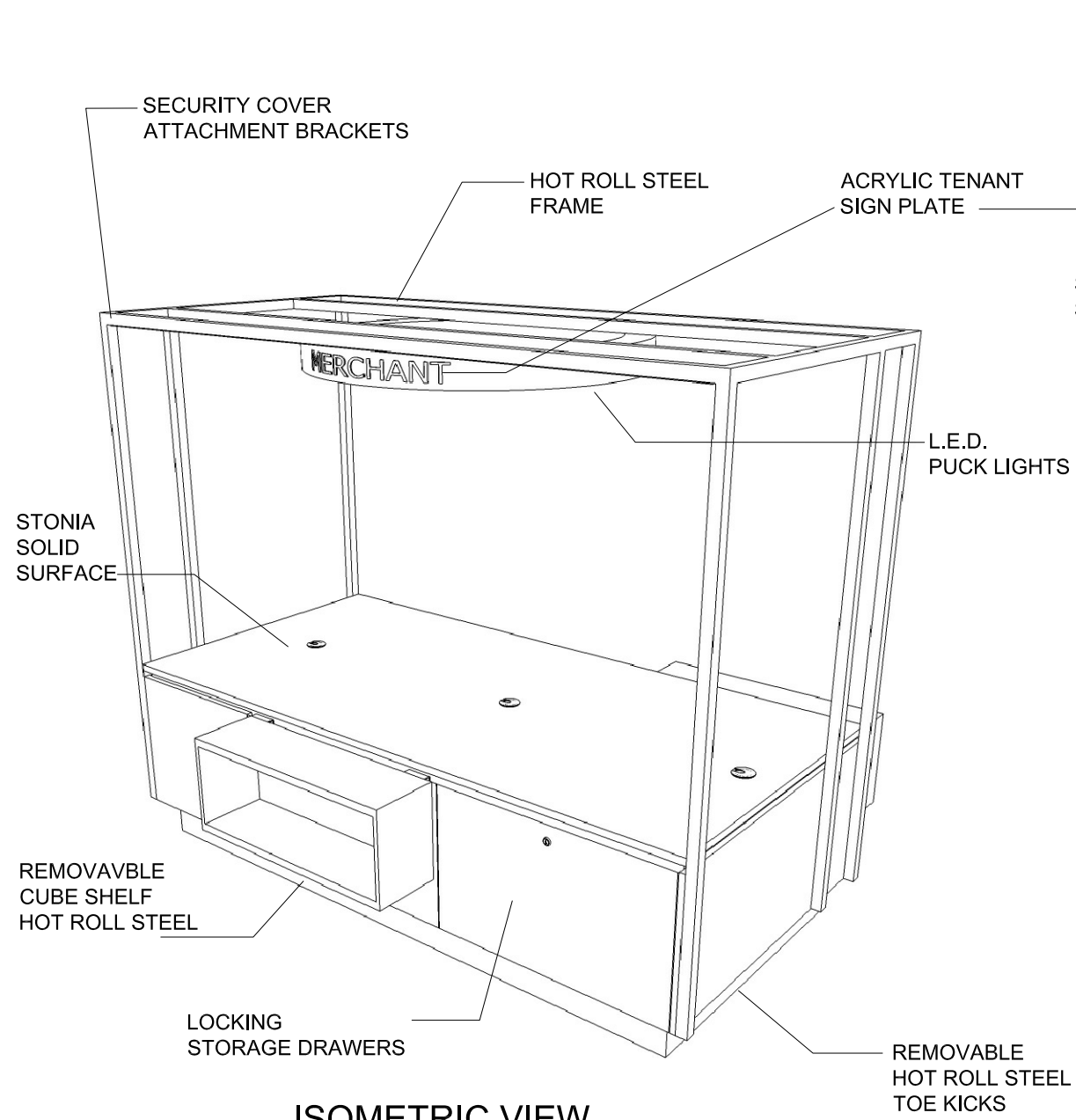
ISOMETRIC VIEW
