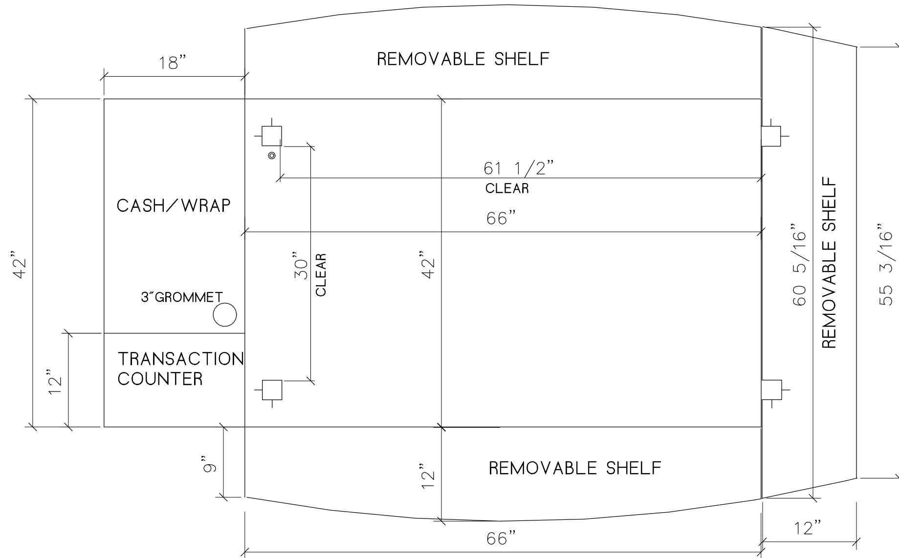
PLAN - COUNTER TOP / COUNTER SHELVES
