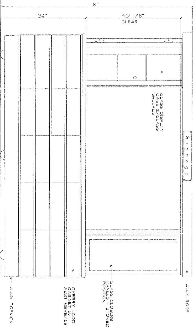
FRONT ELEVATION NORTH BRIDGE RYU Sand Mountain, Inc. - 6/1/04
