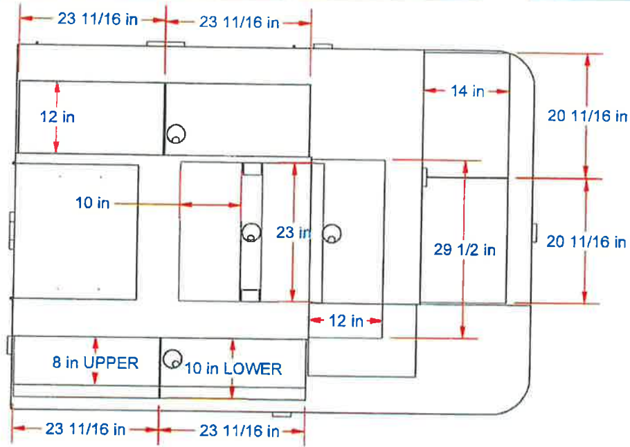
PLAN VIEW GLASS SHELVES
