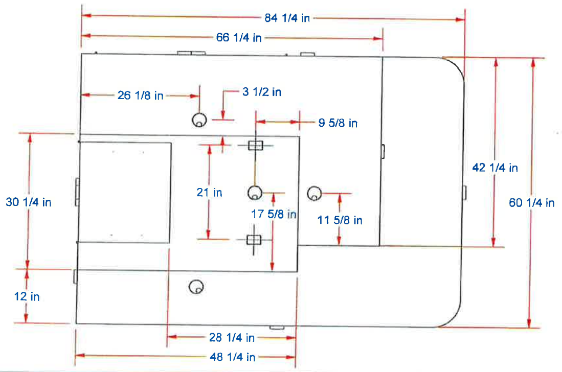
PLAN VIEW COUNTER TOP
