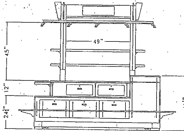
MERCHANDISING DIAGRAM - SIDE ELEVATION SCALE 1/2" = 1'-0"
