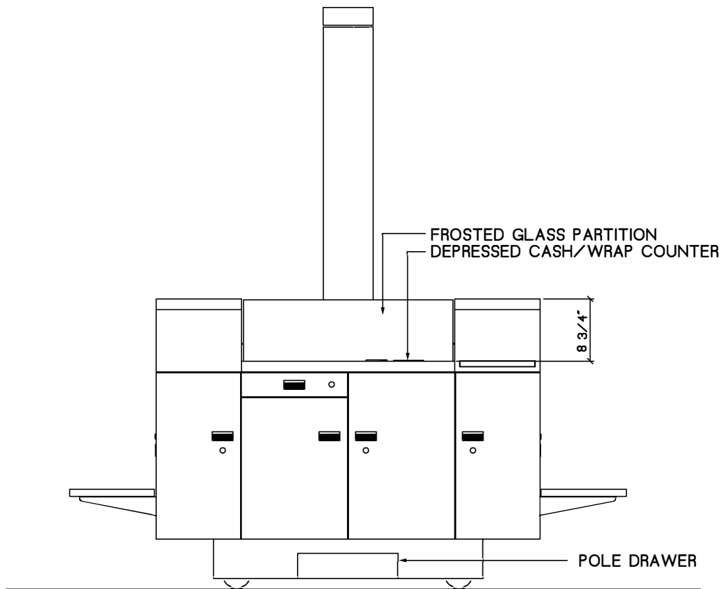
CASH/WRAPELEVATION CP-10 LARGE RMU Sand Mountain, Inc. 5-1-10
