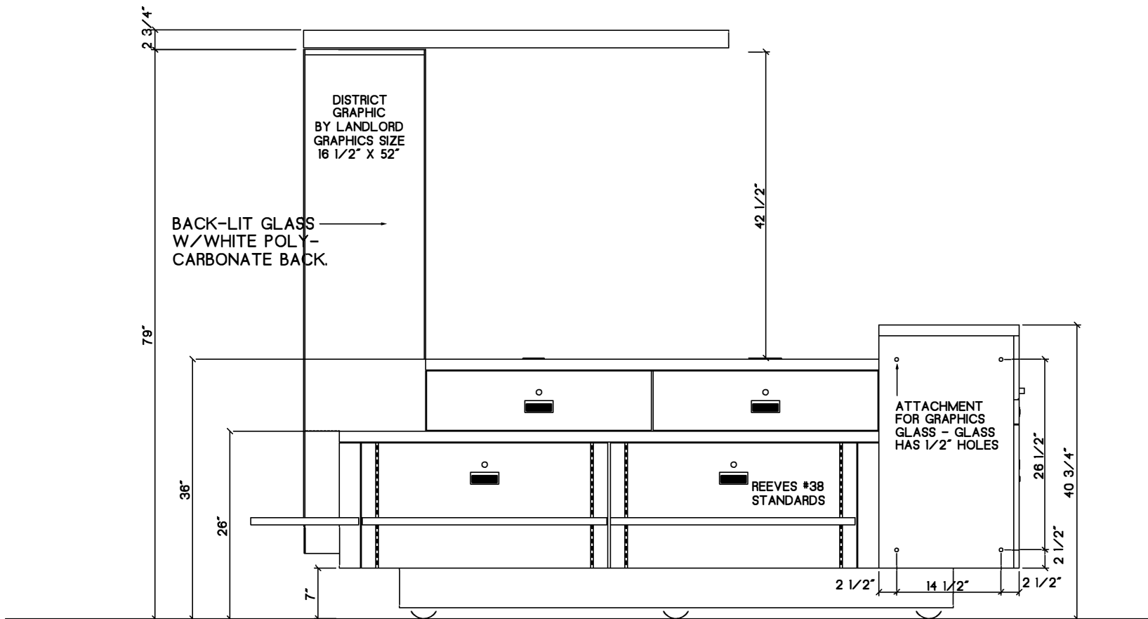
SIDE ELEVATION CP-10 LARGE RMU Sand Mountain, Inc. 5-1-10
