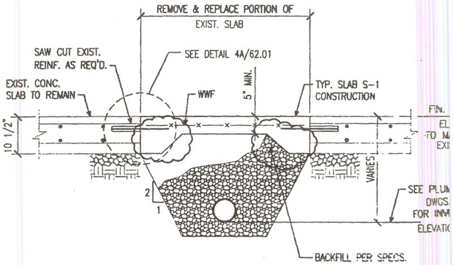
4C SECTION 0 3" 6" 1' 2' 3' SCALE: 3/4" = 1'-0"
