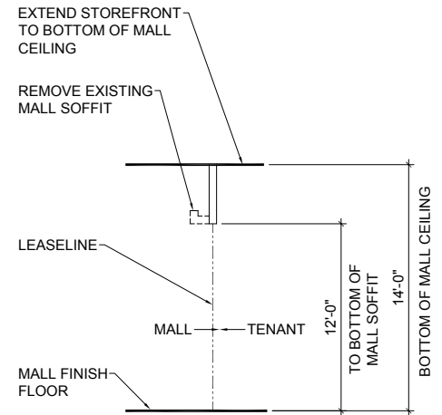
TYPICAL SECTION DETAIL
