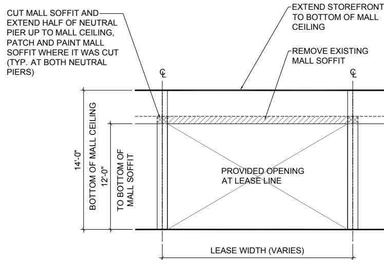
TYPICAL ELEVATION DETAIL
