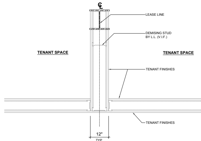
TYPICAL NEUTRAL PIER DETAIL
