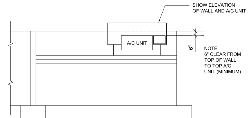
BUILDING SECTION:
