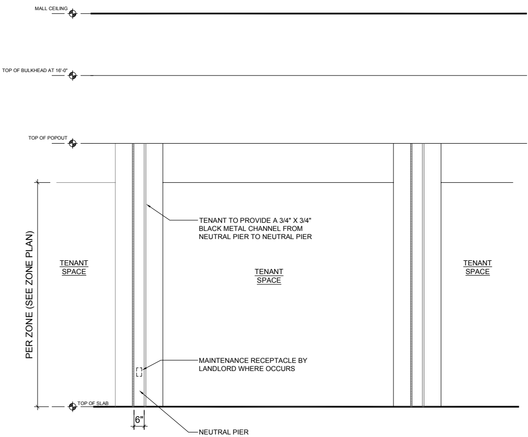
TYPICAL ELEVATION DETAIL CONTACT MALL T.C. FOR MORE INFORMATION - N.T.S.
