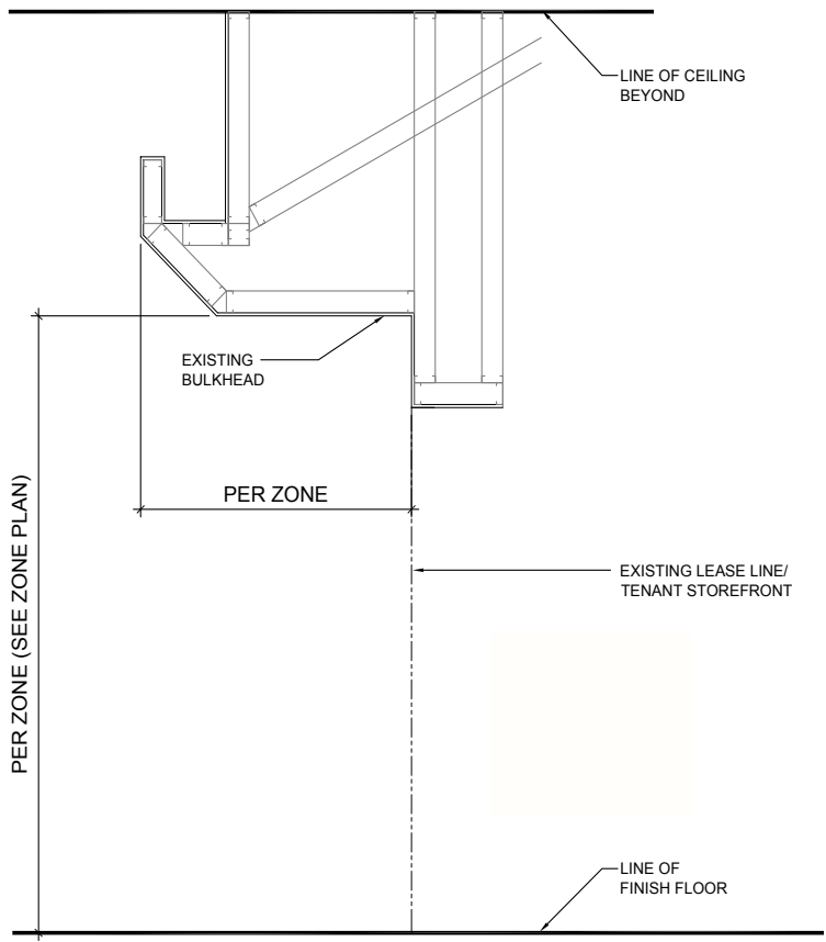
TYPICAL SECTION DETAIL CONTACT MALL T.C. FOR MORE INFORMATION - N.T.S.
