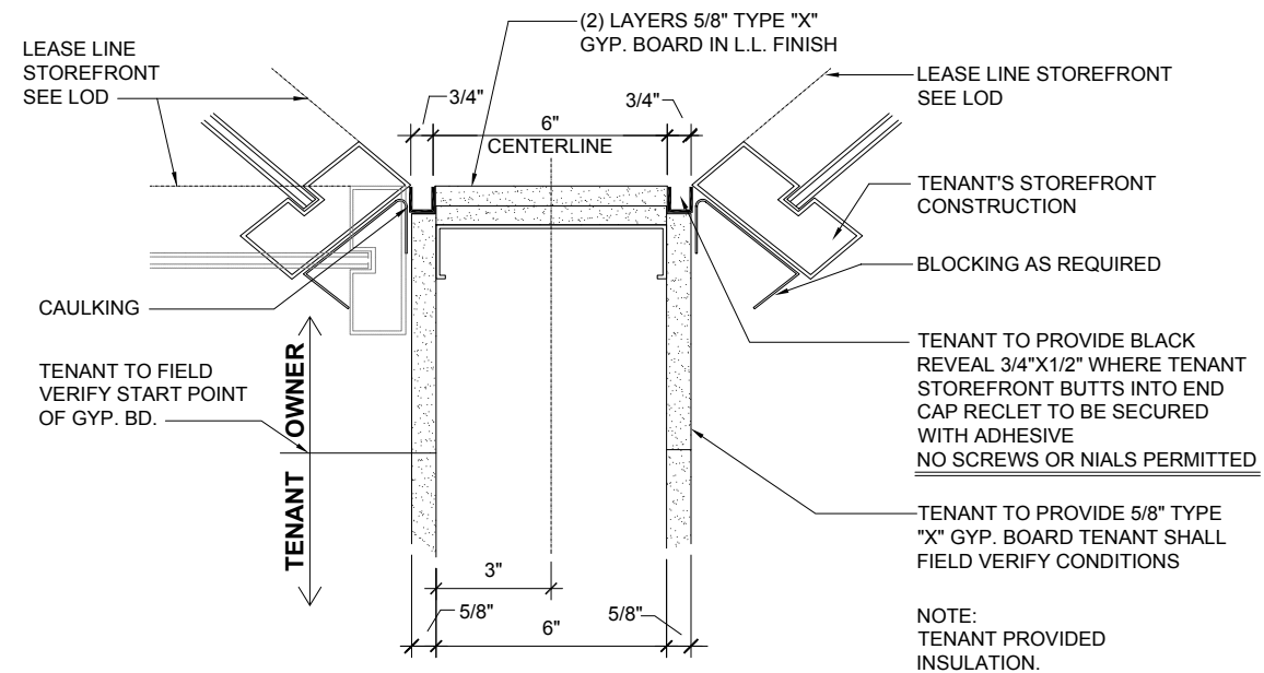
TYPICAL NEUTRAL PIER DETAIL
