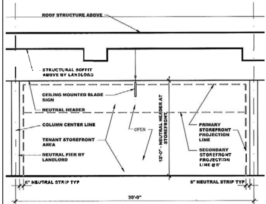
TENANT STOREFRONT ZONES - ZONE 6 - LEVEL TWO STOREFRONT ELEVATION
