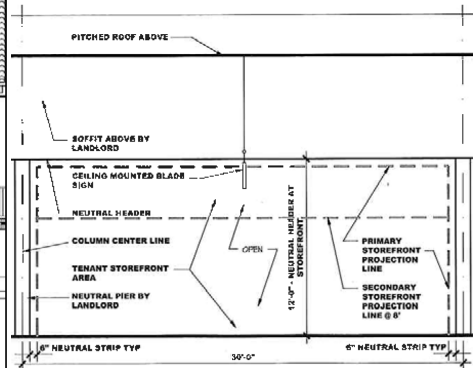
TENANT STOREFRONT ZONES - ZONE 5 - LEVEL TWO STOREFRONT ELEVATION
