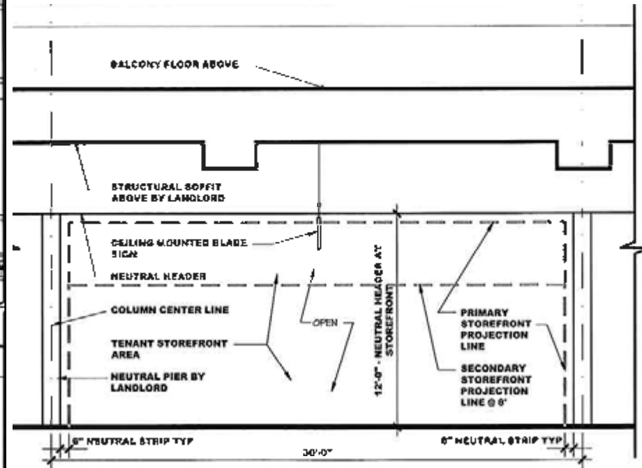
TENANT STOREFRONT ZONES - ZONE 1 - LEVEL ONE STOREFRONT ELEVATION
