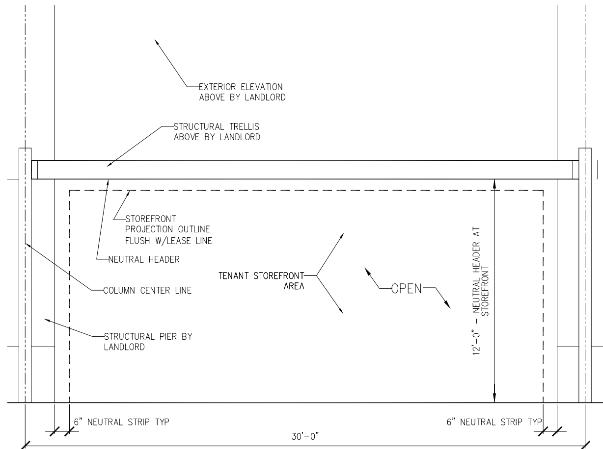
TENANT STOREFRONT ZONES - ZONE 7 - LEVEL TWO BUILDING ELEVATION
