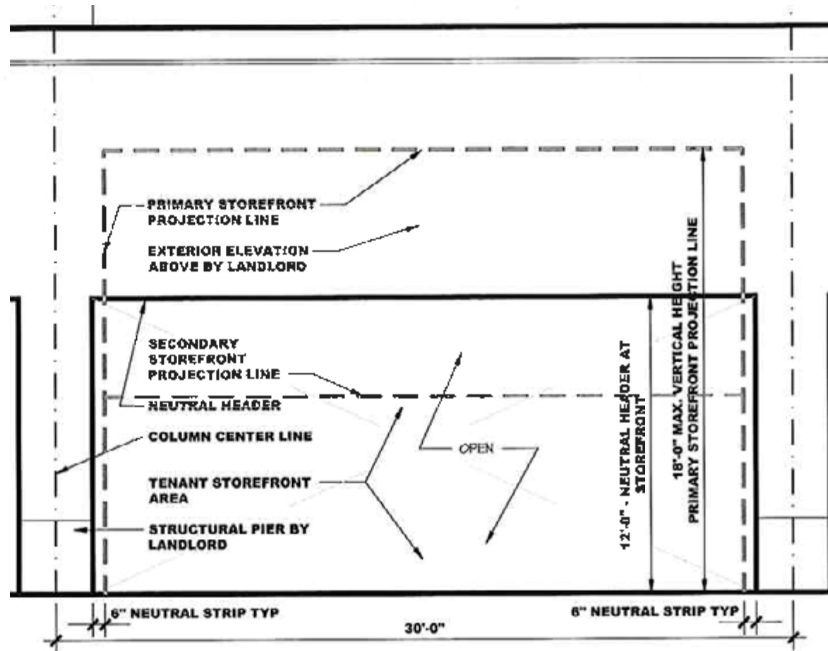
TENANT STOREFRONT ZONES - ZONE 4 - LEVEL TWO STOREFRONT ELEVATION
