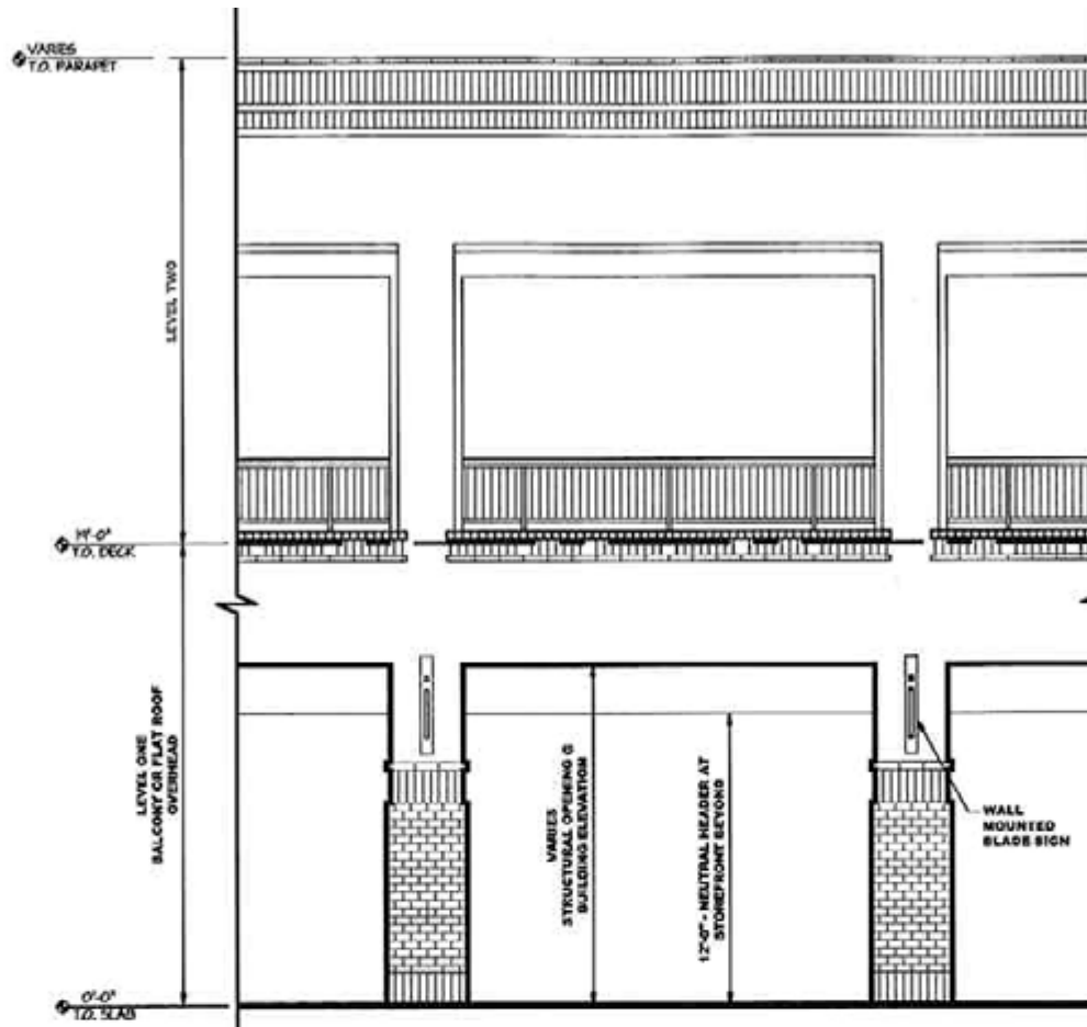
TENANT STOREFRONT ZONES - ZONE 1 - LEVEL ONE BUILDING ELEVATION
