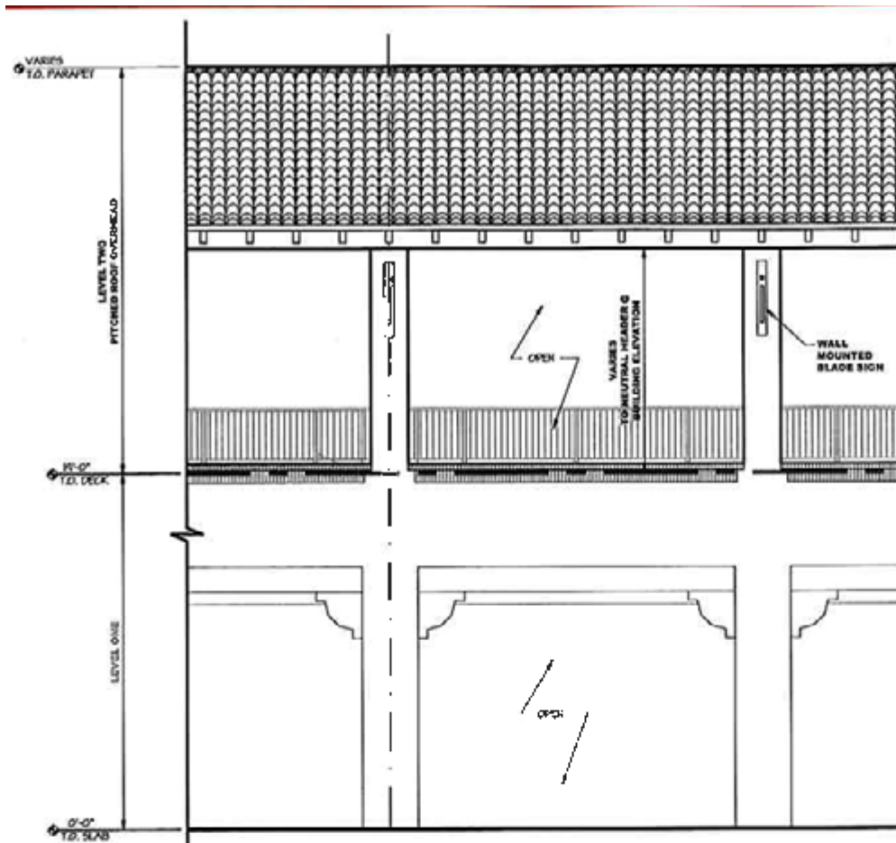
TENANT STOREFRONT ZONES - ZONE 5 - LEVEL TWO BUILDING ELEVATION
