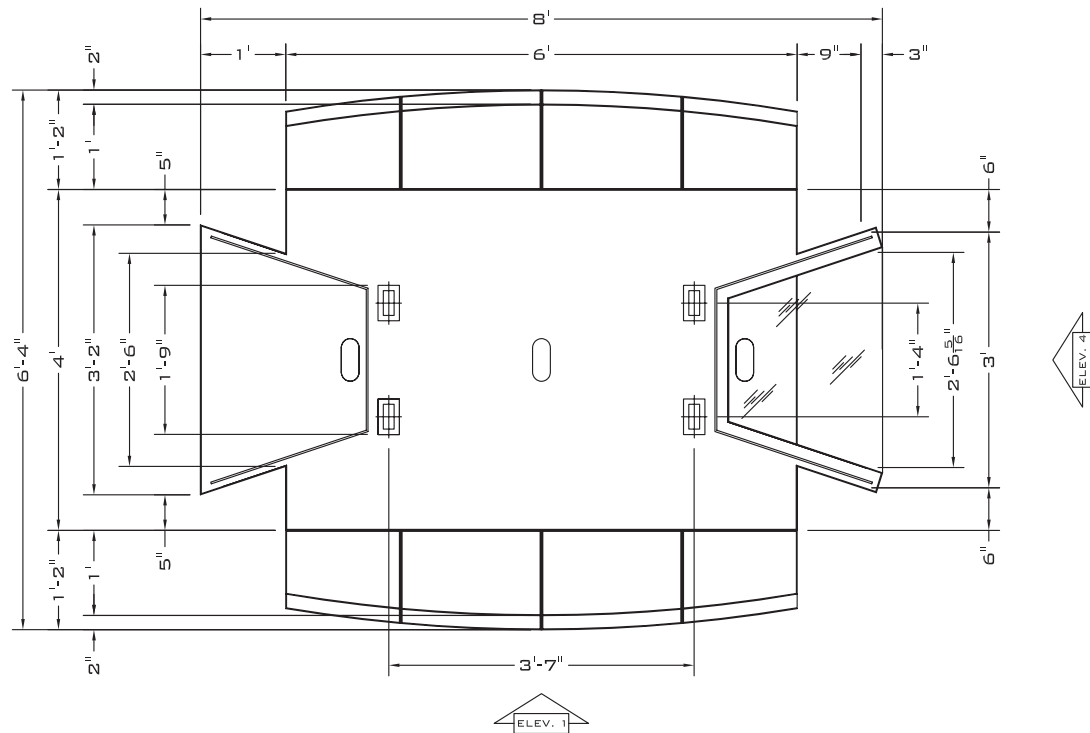
PLAN PLAN @ COUNTER TOP 1 SCALE: 3/4"=1'-0"
