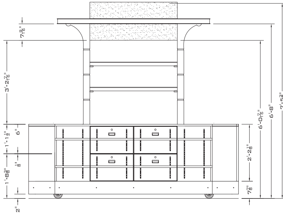
ELEV 1 FRONT ELEVATION SCALE: 3/4"=1'-0"
